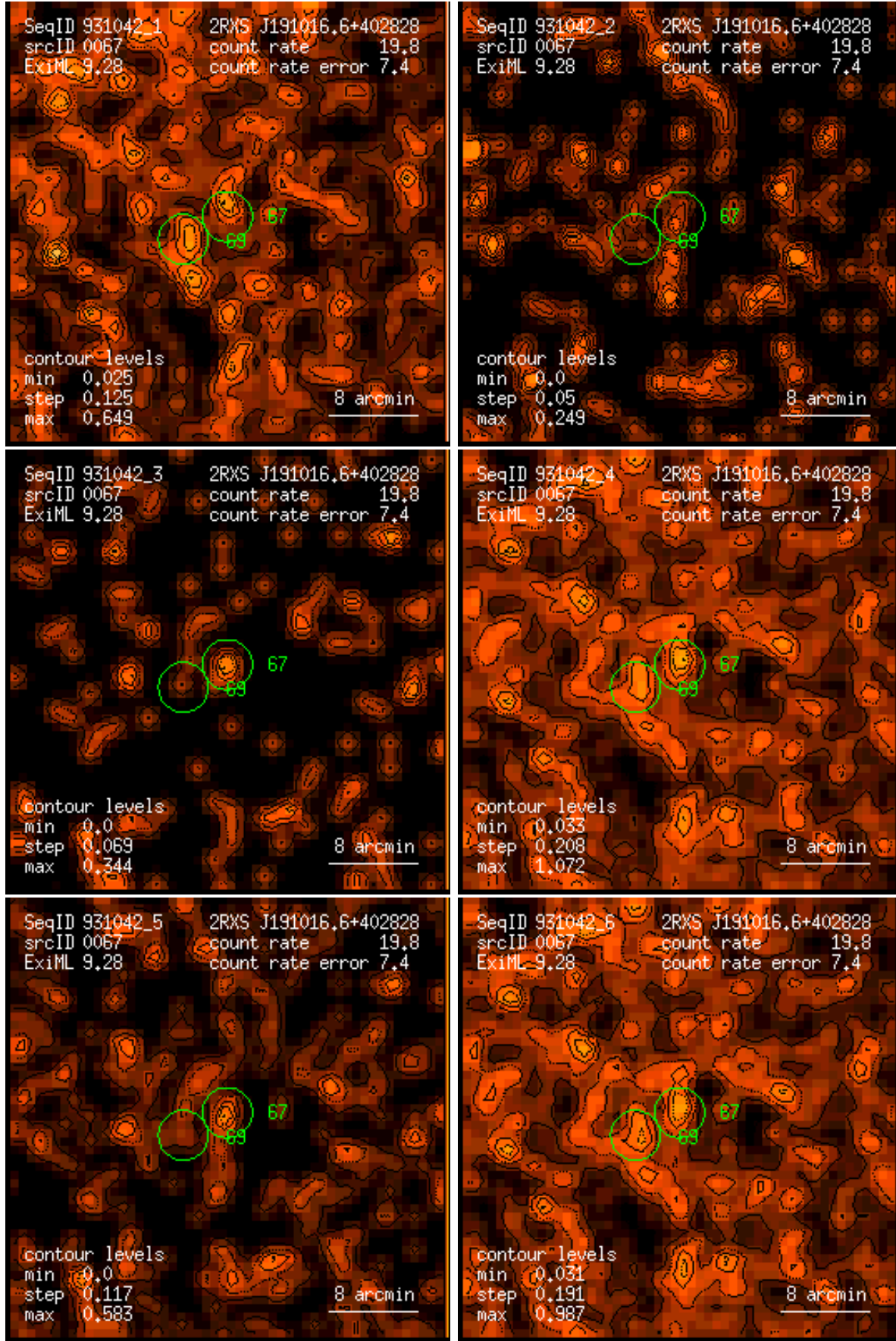
Figure 67: RASS 931042: detection 0067: band rate images, Gaussian filter: (1) PSPC channels 11 – 41, (2) 52 – 90, (3) 91 – 201, (4) 11 – 235, (5) 52 – 201, (6) 11 – 201. Broad band rates in counts/ks. Band rate contour levels in counts/ks/arcmin 2 .
