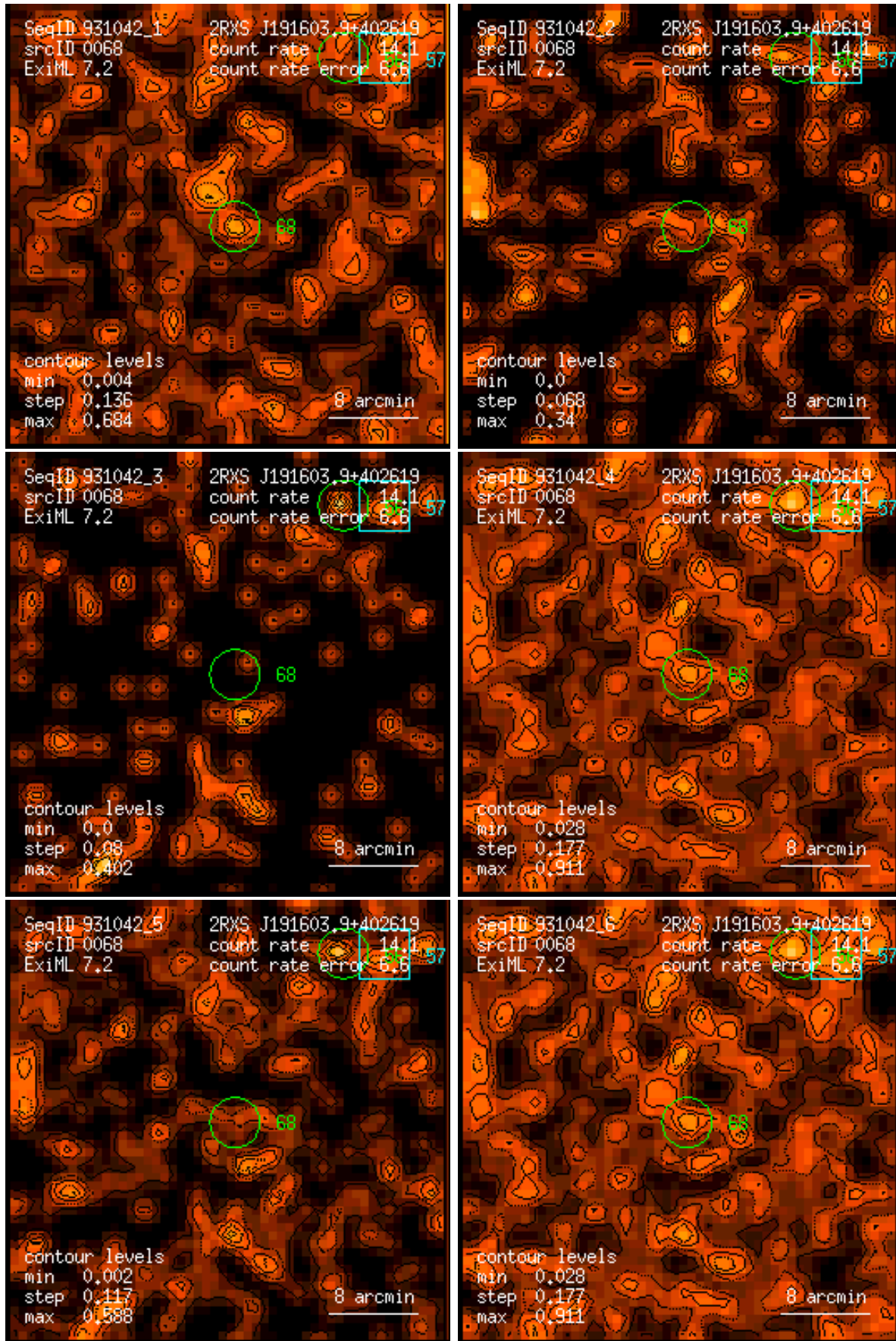
Figure 68: RASS 931042: detection 0068: band rate images, Gaussian filter: (1) PSPC channels 11 – 41, (2) 52 – 90, (3) 91 – 201, (4) 11 – 235, (5) 52 – 201, (6) 11 – 201. Broad band rates in counts/ks. Band rate contour levels in counts/ks/arcmin 2 .
