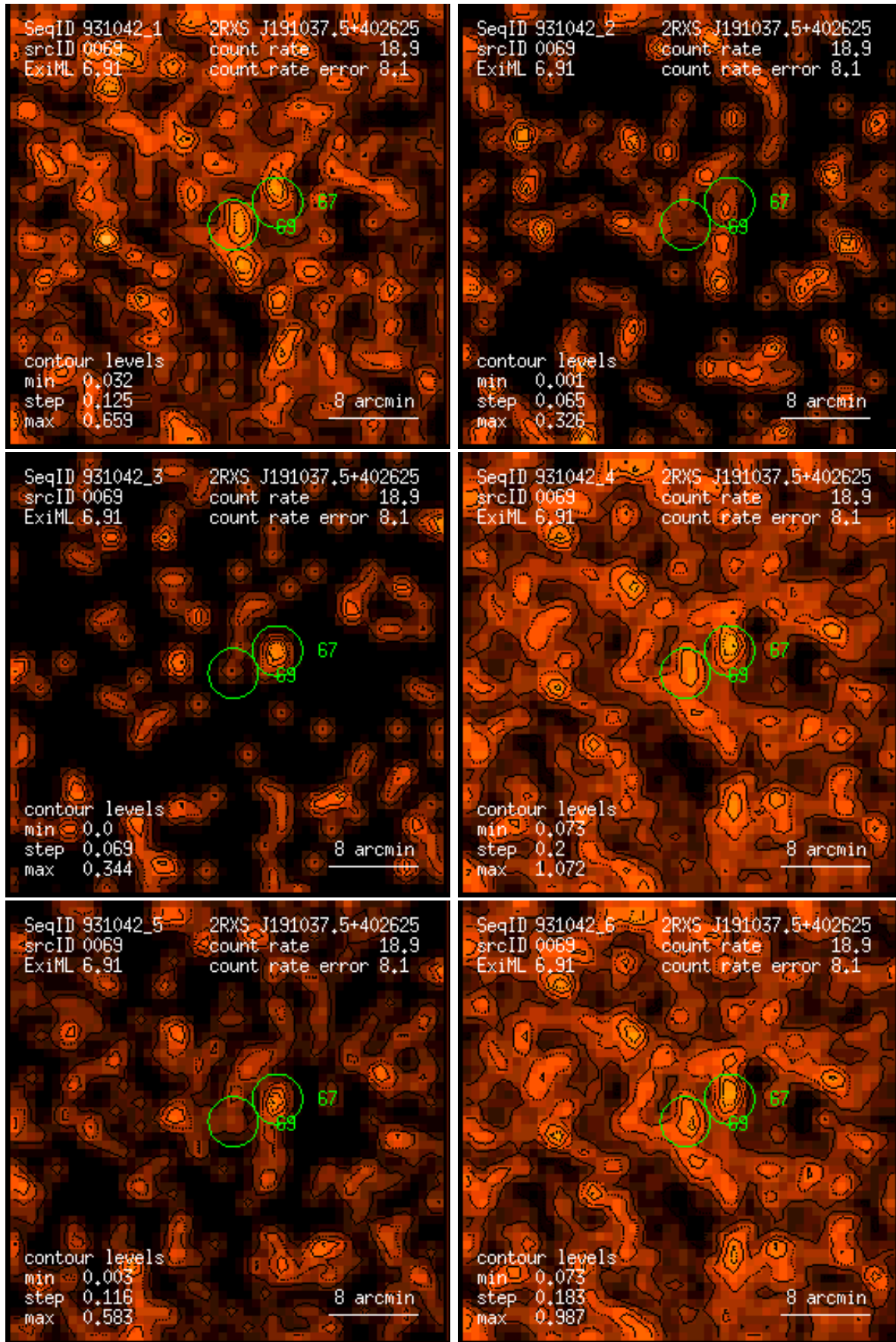
Figure 69: RASS 931042: detection 0069: band rate images, Gaussian filter: (1) PSPC channels 11 – 41, (2) 52 – 90, (3) 91 – 201, (4) 11 – 235, (5) 52 – 201, (6) 11 – 201. Broad band rates in counts/ks. Band rate contour levels in counts/ks/arcmin 2 .
