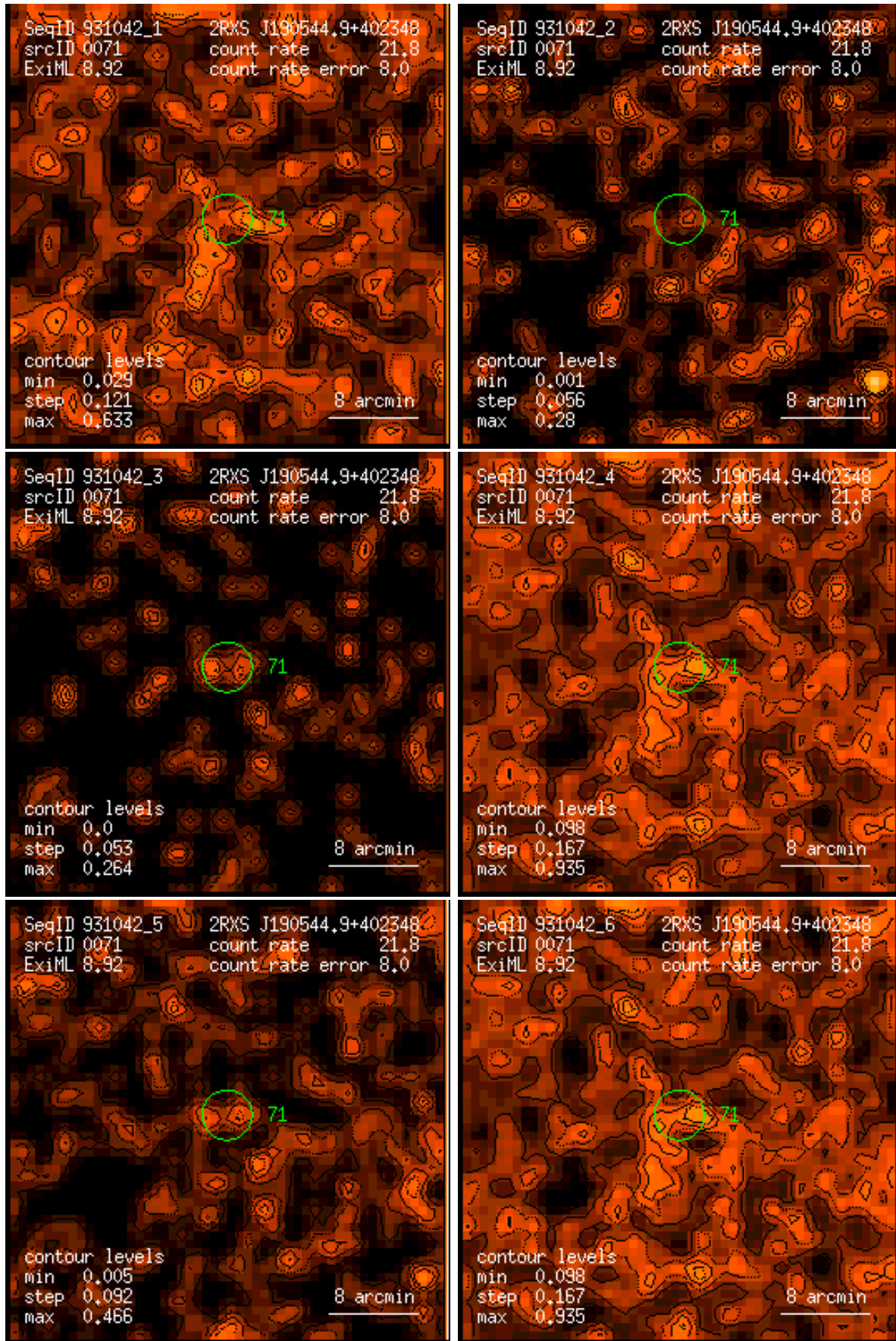
Figure 71: RASS 931042: detection 0071: band rate images, Gaussian filter: (1) PSPC channels 11 – 41, (2) 52 – 90, (3) 91 – 201, (4) 11 – 235, (5) 52 – 201, (6) 11 – 201. Broad band rates in counts/ks. Band rate contour levels in counts/ks/arcmin 2 .
