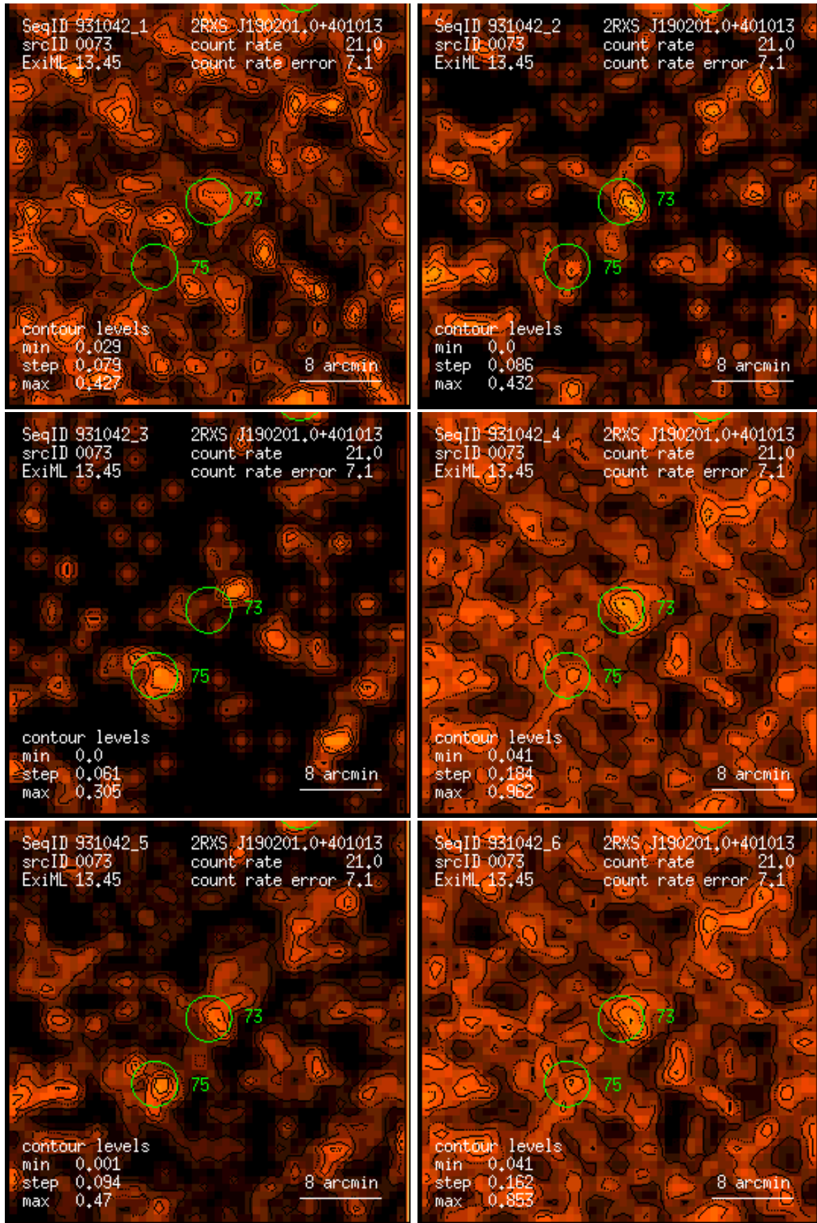
Figure 73: RASS 931042: detection 0073: band rate images, Gaussian filter: (1) PSPC channels 11 – 41, (2) 52 – 90, (3) 91 – 201, (4) 11 – 235, (5) 52 – 201, (6) 11 – 201. Broad band rates in counts/ks. Band rate contour levels in counts/ks/arcmin 2 .
