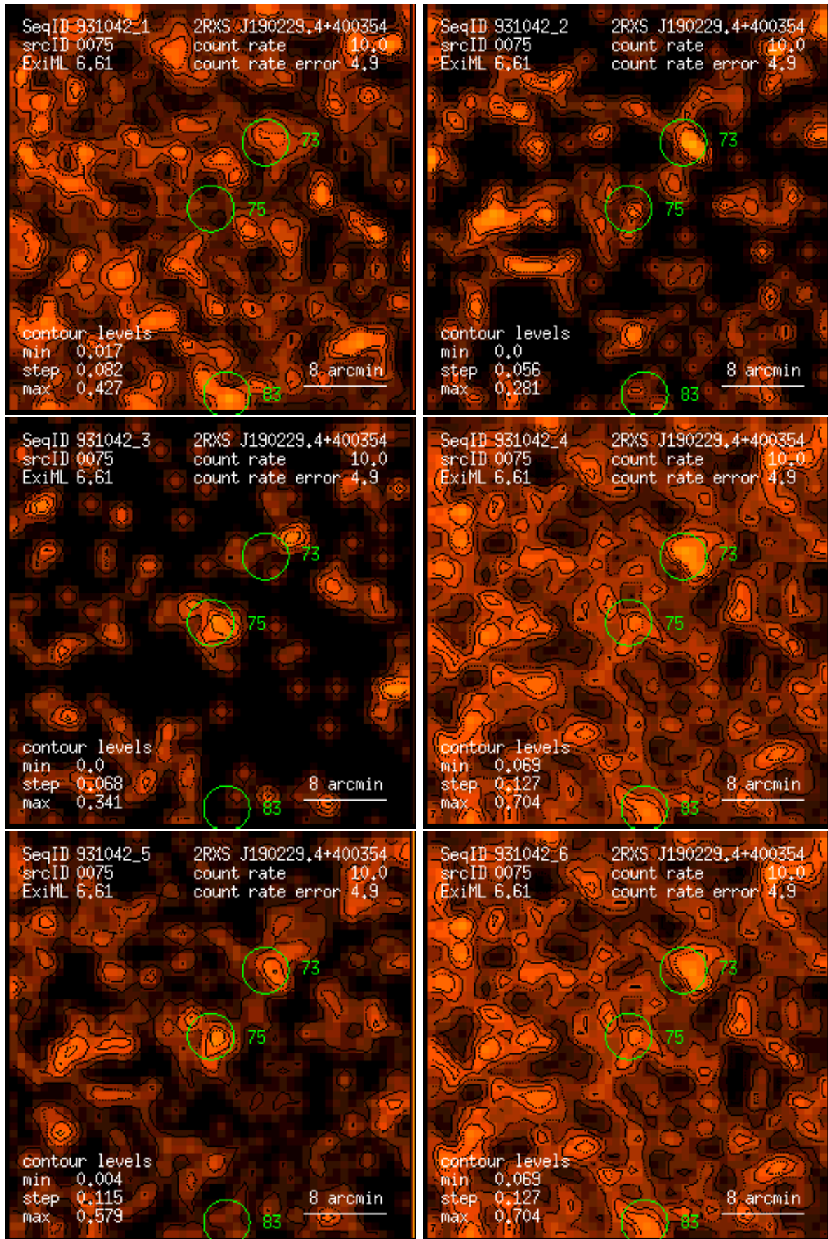
Figure 75: RASS 931042: detection 0075: band rate images, Gaussian filter: (1) PSPC channels 11 – 41, (2) 52 – 90, (3) 91 – 201, (4) 11 – 235, (5) 52 – 201, (6) 11 – 201. Broad band rates in counts/ks. Band rate contour levels in counts/ks/arcmin 2 .
