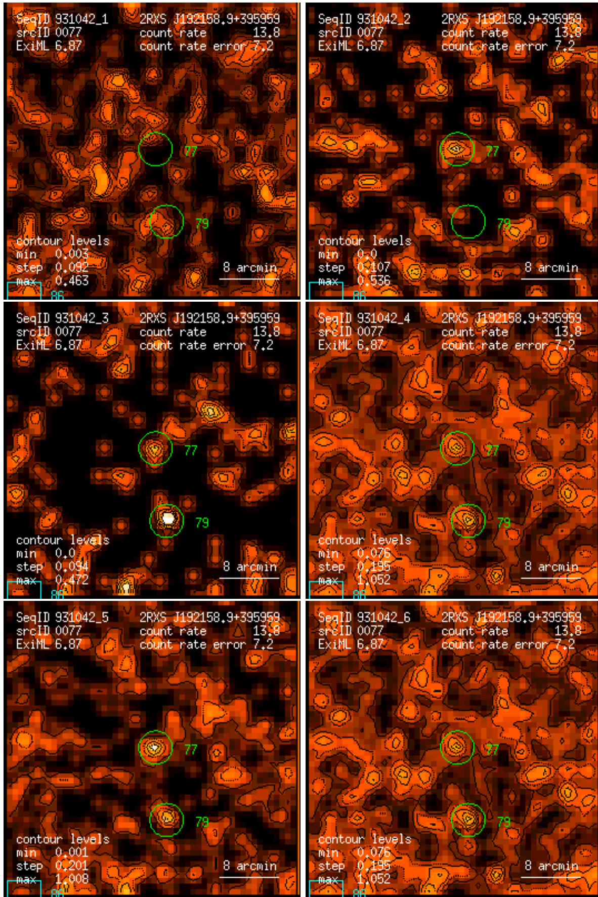
Figure 77: RASS 931042: detection 0077: band rate images, Gaussian filter: (1) PSPC channels 11 – 41, (2) 52 – 90, (3) 91 – 201, (4) 11 – 235, (5) 52 – 201, (6) 11 – 201. Broad band rates in counts/ks. Band rate contour levels in counts/ks/arcmin 2 .
