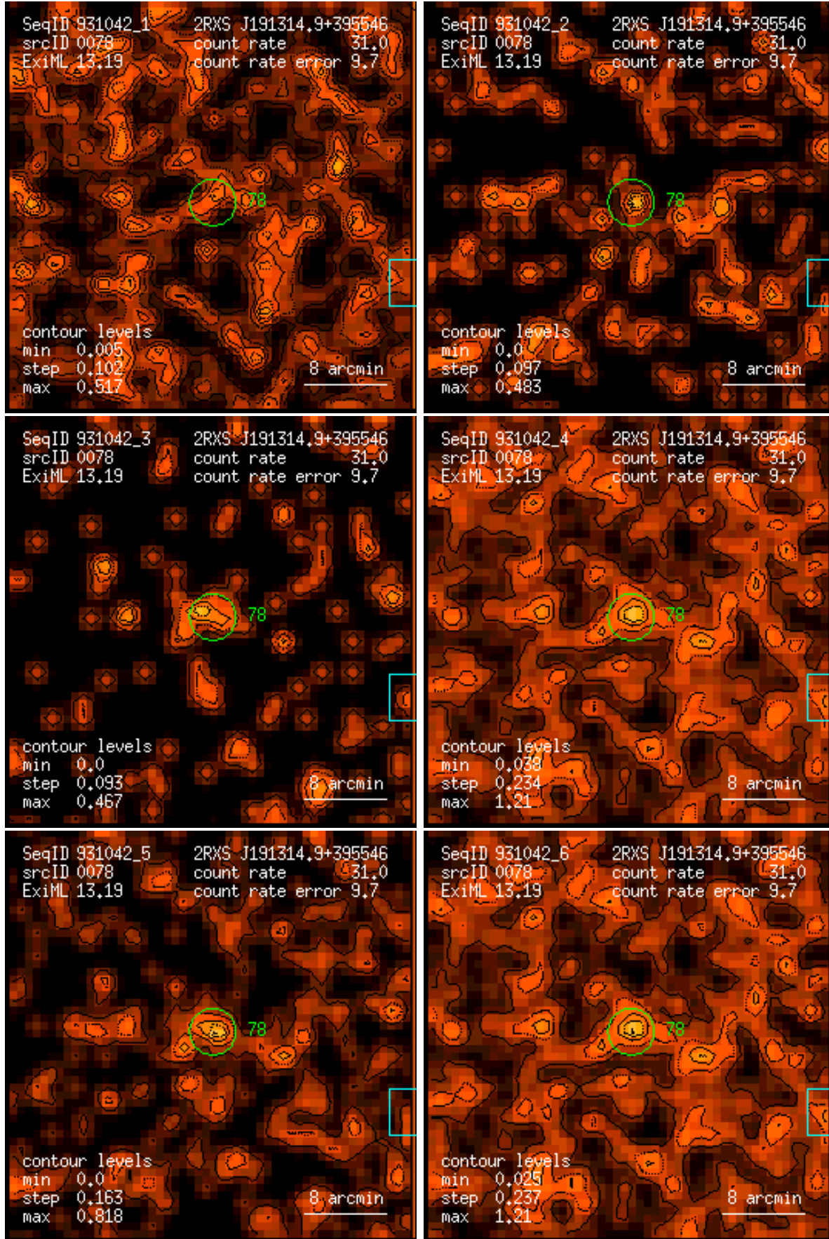
Figure 78: RASS 931042: detection 0078: band rate images, Gaussian filter: (1) PSPC channels 11 – 41, (2) 52 – 90, (3) 91 – 201, (4) 11 – 235, (5) 52 – 201, (6) 11 – 201. Broad band rates in counts/ks. Band rate contour levels in counts/ks/arcmin 2 .
