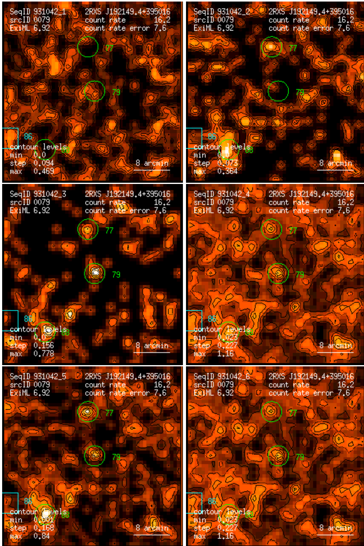
Figure 79: RASS 931042: detection 0079: band rate images, Gaussian filter: (1) PSPC channels 11 – 41, (2) 52 – 90, (3) 91 – 201, (4) 11 – 235, (5) 52 – 201, (6) 11 – 201. Broad band rates in counts/ks. Band rate contour levels in counts/ks/arcmin 2 .
