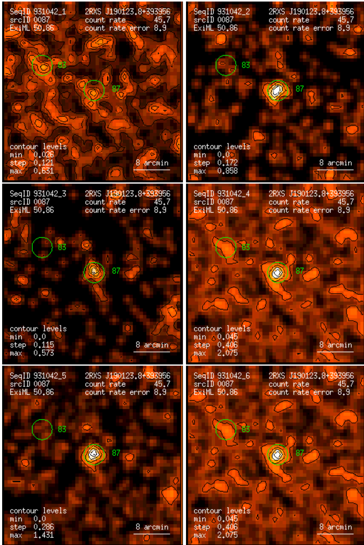
Figure 87: RASS 931042: detection 0087: band rate images, Gaussian filter: (1) PSPC channels 11 – 41, (2) 52 – 90, (3) 91 – 201, (4) 11 – 235, (5) 52 – 201, (6) 11 – 201. Broad band rates in counts/ks. Band rate contour levels in counts/ks/arcmin 2 .
