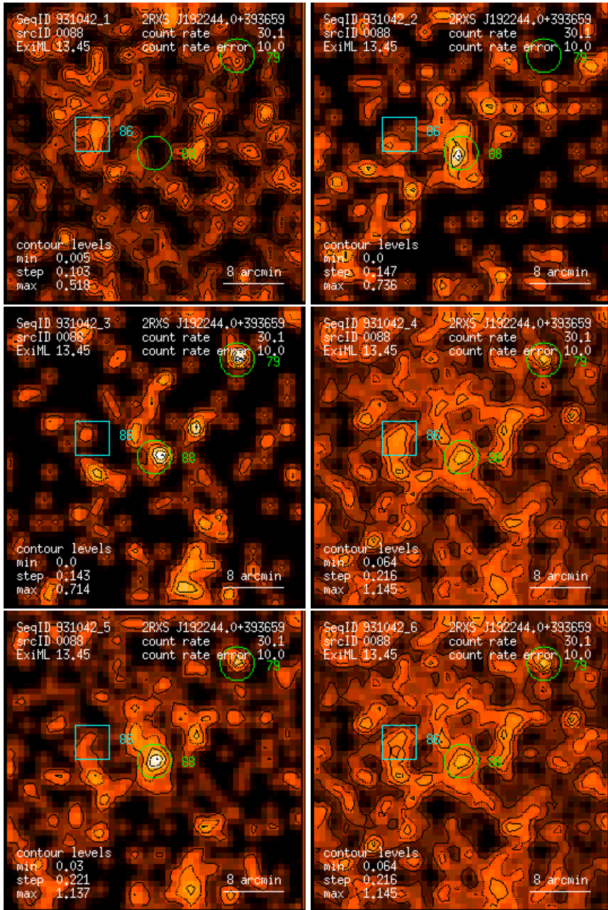
Figure 88: RASS 931042: detection 0088: band rate images, Gaussian filter: (1) PSPC channels 11 – 41, (2) 52 – 90, (3) 91 – 201, (4) 11 – 235, (5) 52 – 201, (6) 11 – 201. Broad band rates in counts/ks. Band rate contour levels in counts/ks/arcmin 2 .
