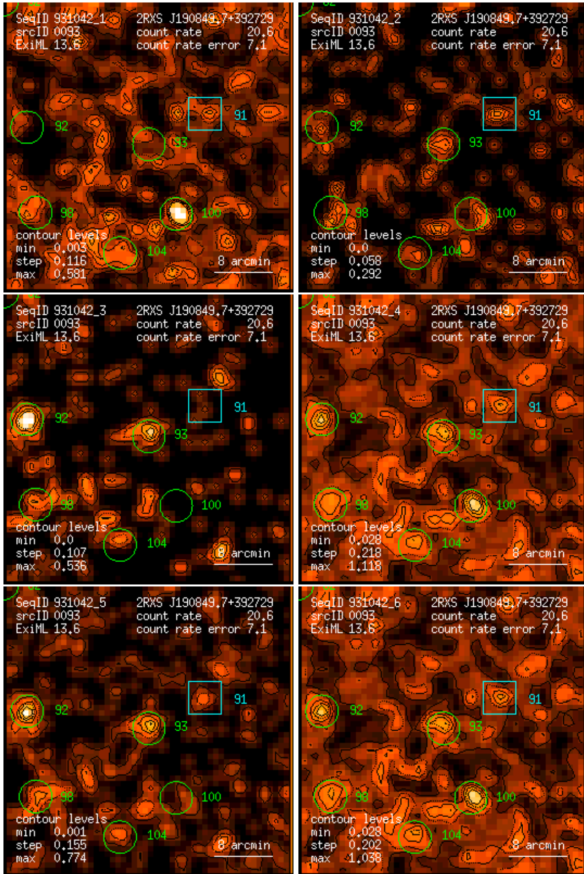
Figure 93: RASS 931042: detection 0093: band rate images, Gaussian filter: (1) PSPC channels 11 – 41, (2) 52 – 90, (3) 91 – 201, (4) 11 – 235, (5) 52 – 201, (6) 11 – 201. Broad band rates in counts/ks. Band rate contour levels in counts/ks/arcmin 2 .
