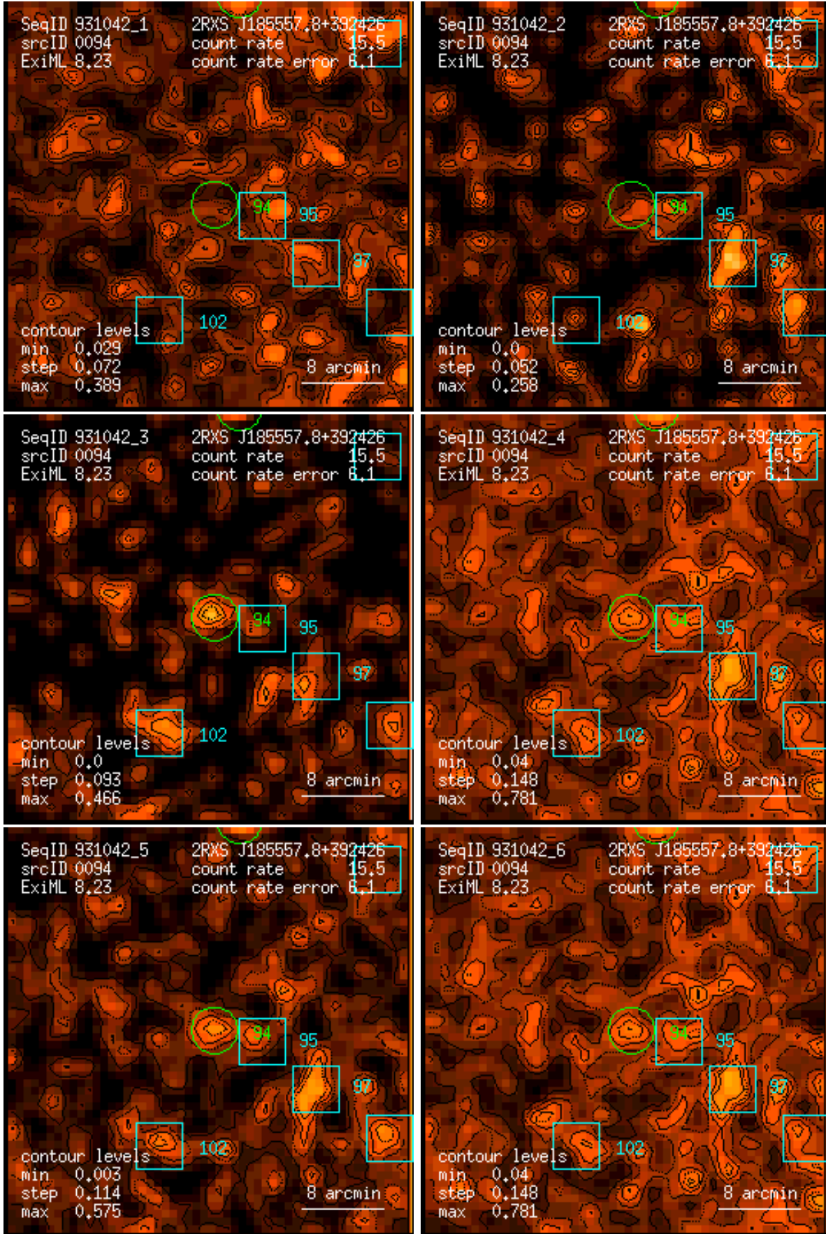
Figure 94: RASS 931042: detection 0094: band rate images, Gaussian filter: (1) PSPC channels 11 – 41, (2) 52 – 90, (3) 91 – 201, (4) 11 – 235, (5) 52 – 201, (6) 11 – 201. Broad band rates in counts/ks. Band rate contour levels in counts/ks/arcmin 2 .
