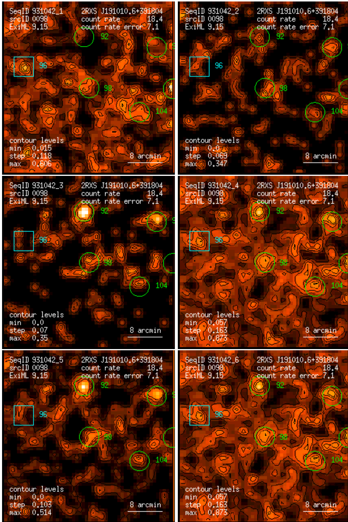
Figure 98: RASS 931042: detection 0098: band rate images, Gaussian filter: (1) PSPC channels 11 – 41, (2) 52 – 90, (3) 91 – 201, (4) 11 – 235, (5) 52 – 201, (6) 11 – 201. Broad band rates in counts/ks. Band rate contour levels in counts/ks/arcmin 2 .
