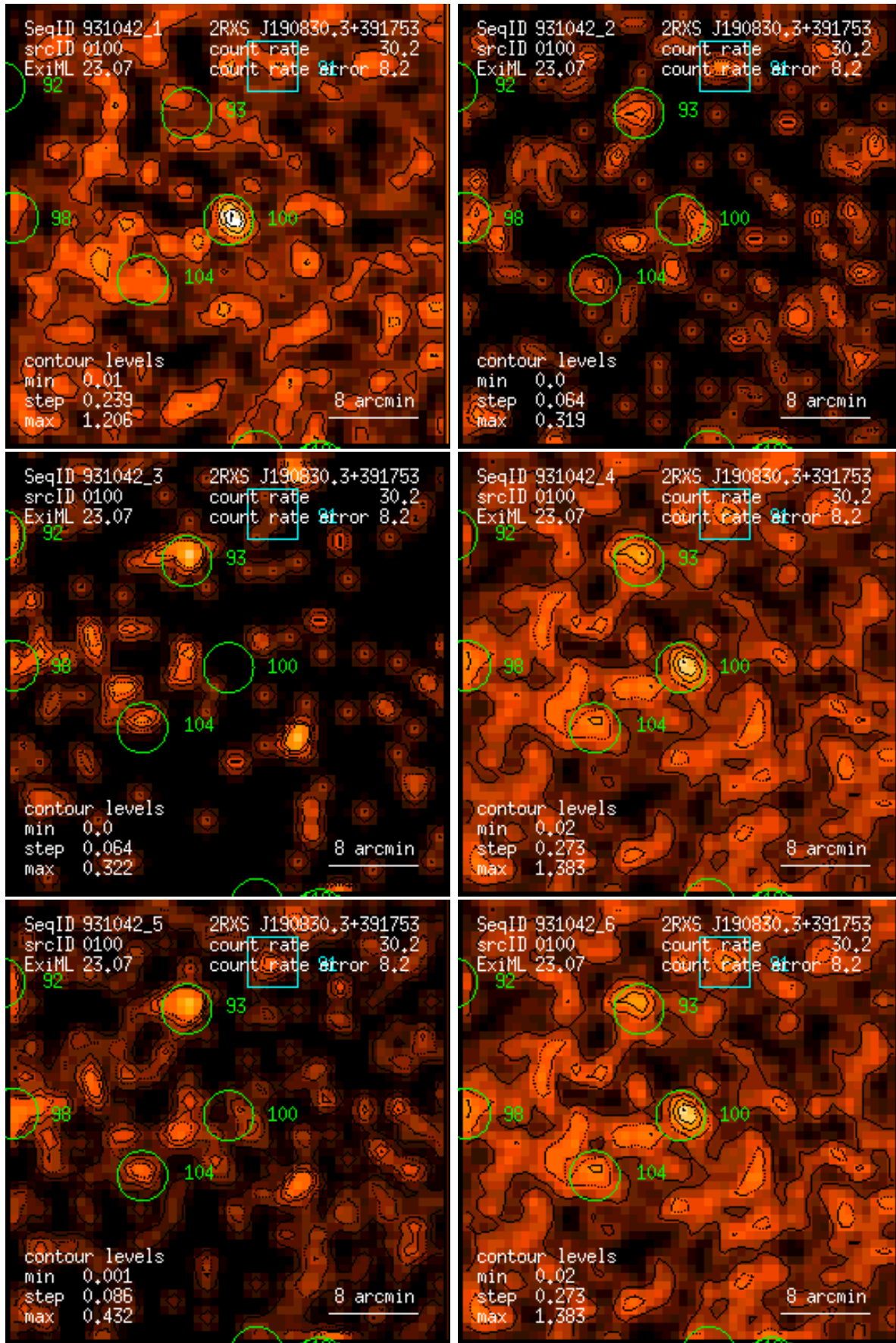
Figure 100: RASS 931042: detection 0100: band rate images, Gaussian filter: (1) PSPC channels 11 – 41, (2) 52 – 90, (3) 91 – 201, (4) 11 – 235, (5) 52 – 201, (6) 11 – 201. Broad band rates in counts/ks. Band rate contour levels in counts/ks/arcmin 2 .
