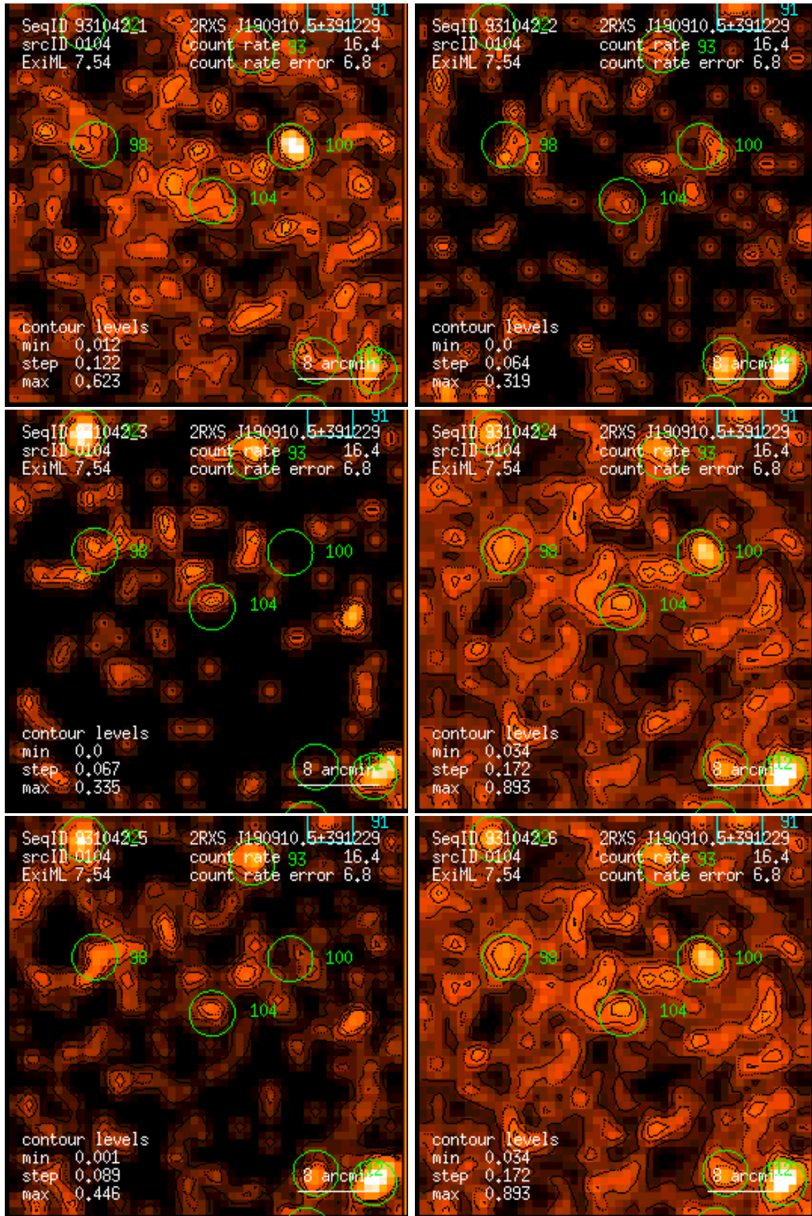
Figure 104: RASS 931042: detection 0104: band rate images, Gaussian filter: (1) PSPC channels 11 – 41, (2) 52 – 90, (3) 91 – 201, (4) 11 – 235, (5) 52 – 201, (6) 11 – 201. Broad band rates in counts/ks. Band rate contour levels in counts/ks/arcmin 2 .
