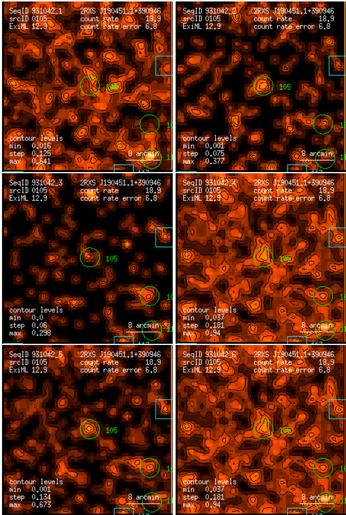
Figure 105: RASS 931042: detection 0105: band rate images, Gaussian filter: (1) PSPC channels 11 – 41, (2) 52 – 90, (3) 91 – 201, (4) 11 – 235, (5) 52 – 201, (6) 11 – 201. Broad band rates in counts/ks. Band rate contour levels in counts/ks/arcmin 2 .
