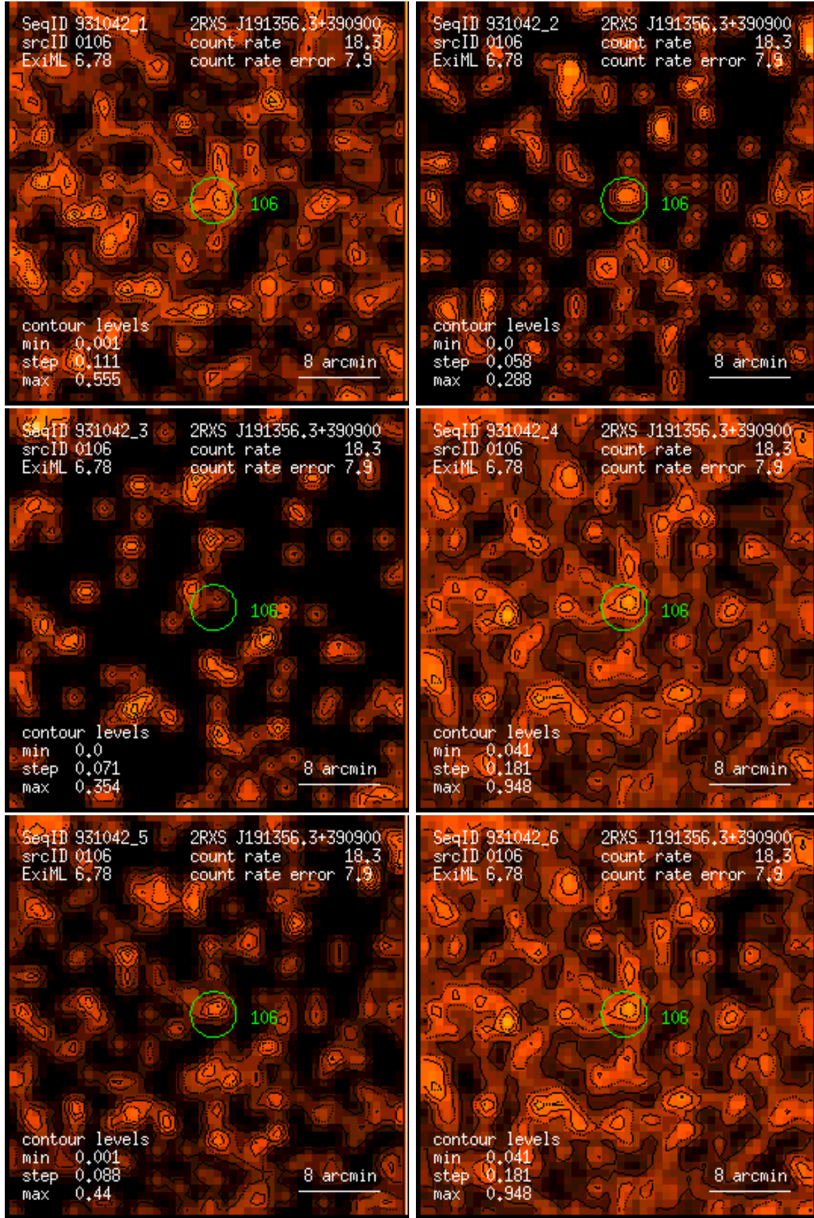
Figure 106: RASS 931042: detection 0106: band rate images, Gaussian filter: (1) PSPC channels 11 – 41, (2) 52 – 90, (3) 91 – 201, (4) 11 – 235, (5) 52 – 201, (6) 11 – 201. Broad band rates in counts/ks. Band rate contour levels in counts/ks/arcmin 2 .
