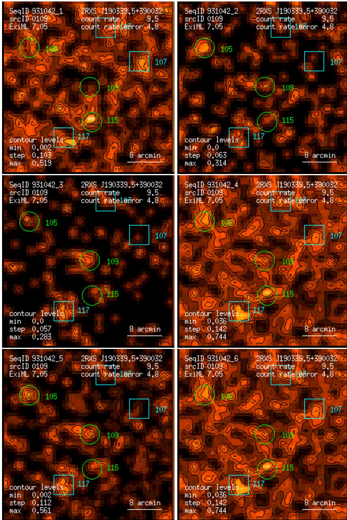
Figure 109: RASS 931042: detection 0109: band rate images, Gaussian filter: (1) PSPC channels 11 – 41, (2) 52 – 90, (3) 91 – 201, (4) 11 – 235, (5) 52 – 201, (6) 11 – 201. Broad band rates in counts/ks. Band rate contour levels in counts/ks/arcmin 2 .
