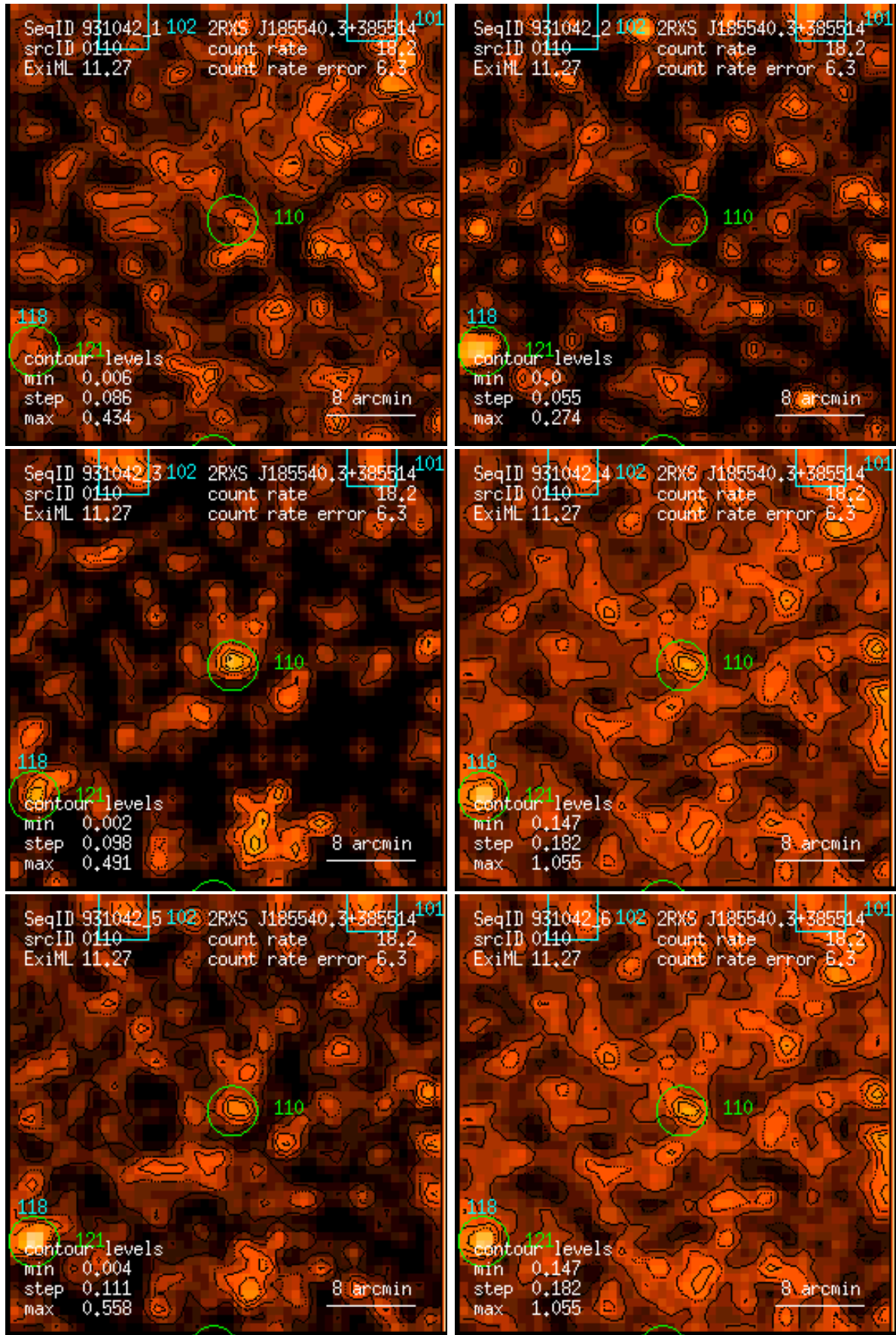
Figure 110: RASS 931042: detection 0110: band rate images, Gaussian filter: (1) PSPC channels 11 – 41, (2) 52 – 90, (3) 91 – 201, (4) 11 – 235, (5) 52 – 201, (6) 11 – 201. Broad band rates in counts/ks. Band rate contour levels in counts/ks/arcmin 2 .
