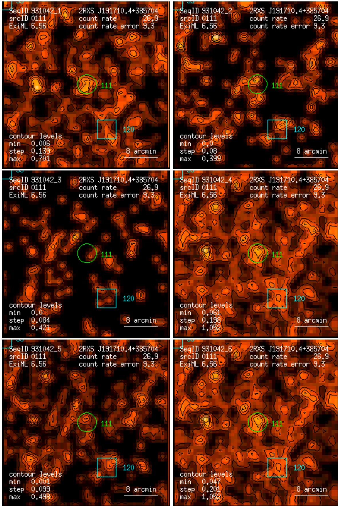
Figure 111: RASS 931042: detection 0111: band rate images, Gaussian filter: (1) PSPC channels 11 – 41, (2) 52 – 90, (3) 91 – 201, (4) 11 – 235, (5) 52 – 201, (6) 11 – 201. Broad band rates in counts/ks. Band rate contour levels in counts/ks/arcmin 2 .
