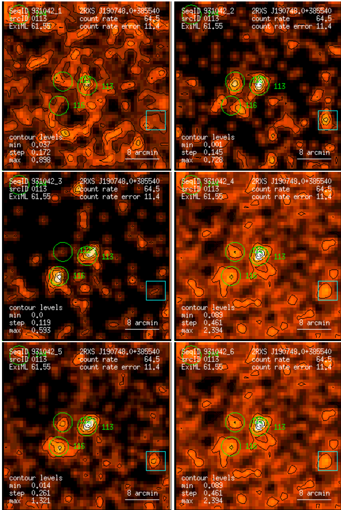
Figure 113: RASS 931042: detection 0113: band rate images, Gaussian filter: (1) PSPC channels 11 – 41, (2) 52 – 90, (3) 91 – 201, (4) 11 – 235, (5) 52 – 201, (6) 11 – 201. Broad band rates in counts/ks. Band rate contour levels in counts/ks/arcmin 2 .
