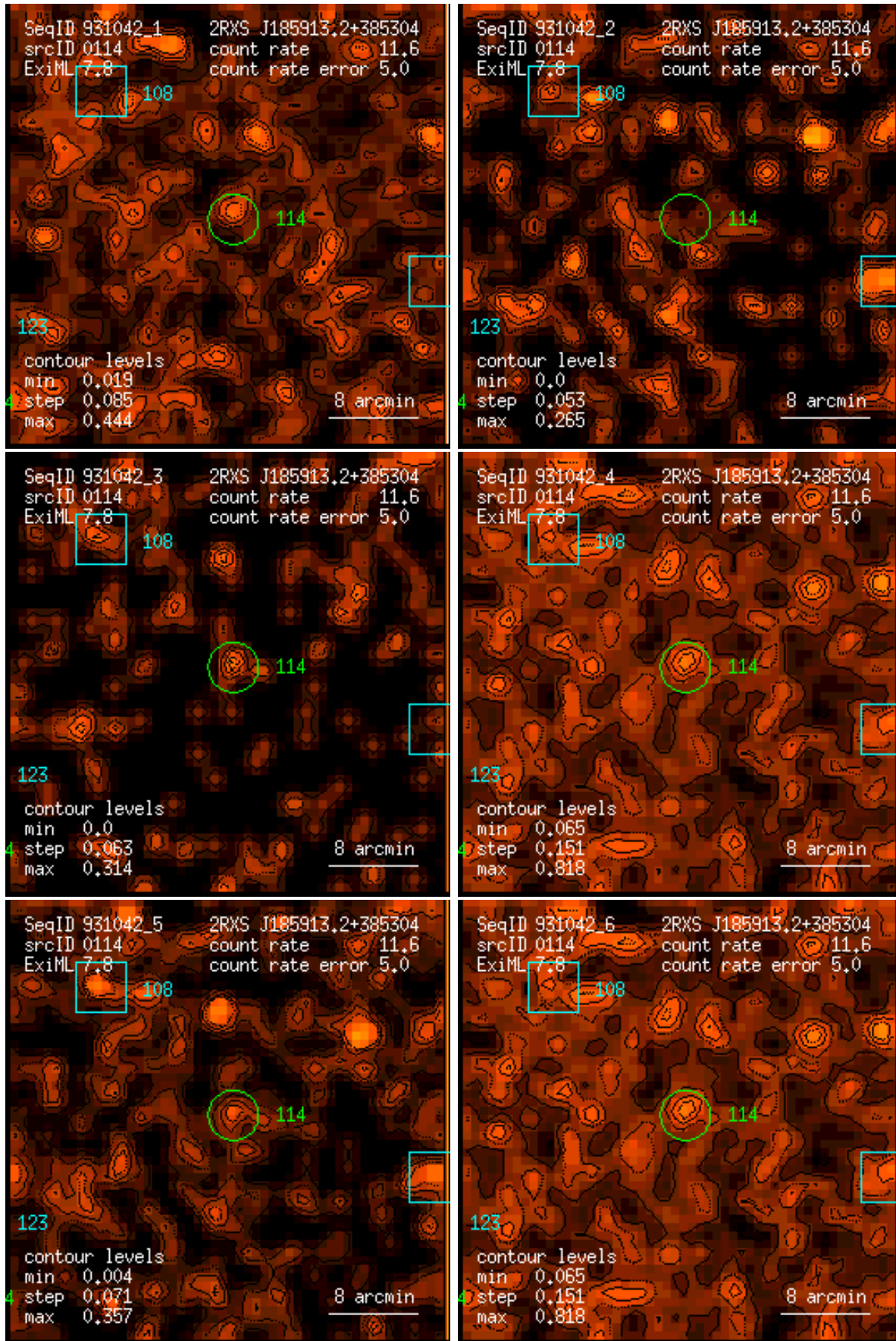
Figure 114: RASS 931042: detection 0114: band rate images, Gaussian filter: (1) PSPC channels 11 – 41, (2) 52 – 90, (3) 91 – 201, (4) 11 – 235, (5) 52 – 201, (6) 11 – 201. Broad band rates in counts/ks. Band rate contour levels in counts/ks/arcmin 2 .
