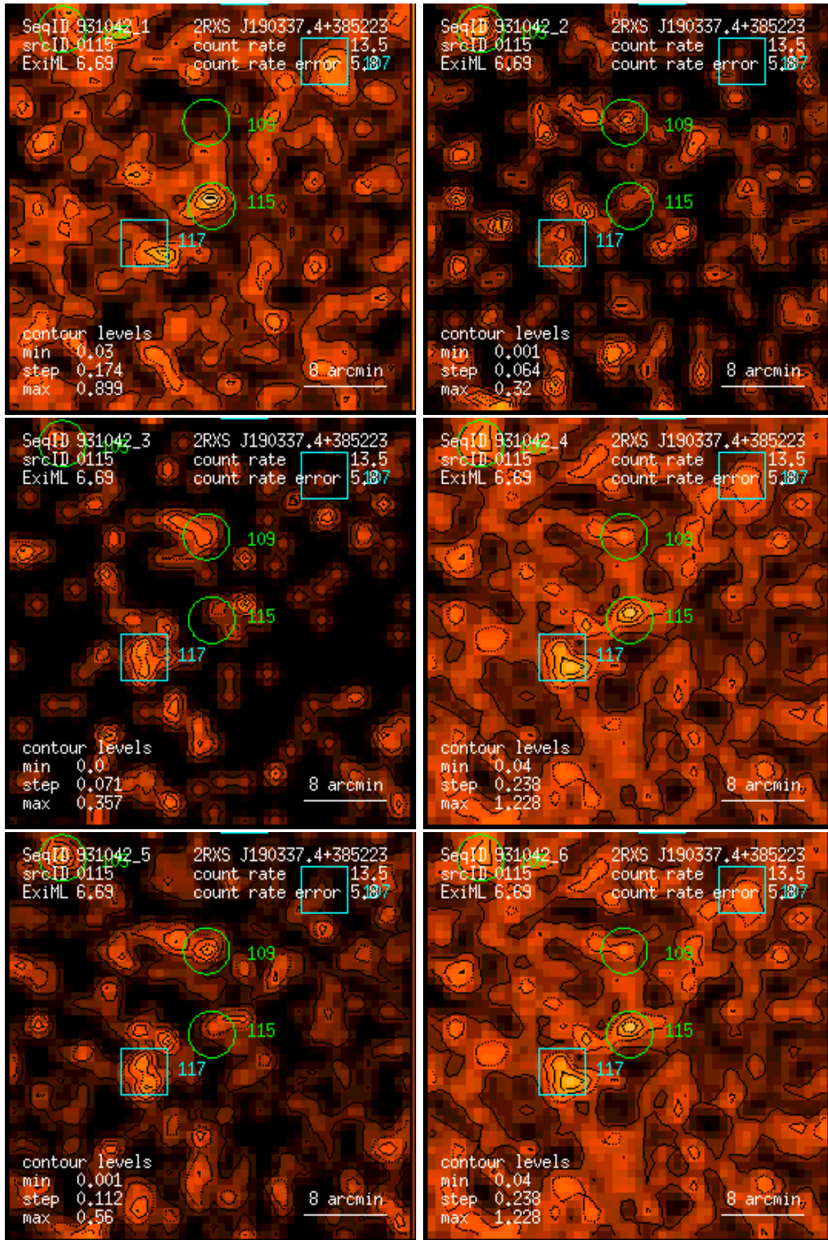
Figure 115: RASS 931042: detection 0115: band rate images, Gaussian filter: (1) PSPC channels 11 – 41, (2) 52 – 90, (3) 91 – 201, (4) 11 – 235, (5) 52 – 201, (6) 11 – 201. Broad band rates in counts/ks. Band rate contour levels in counts/ks/arcmin 2 .
