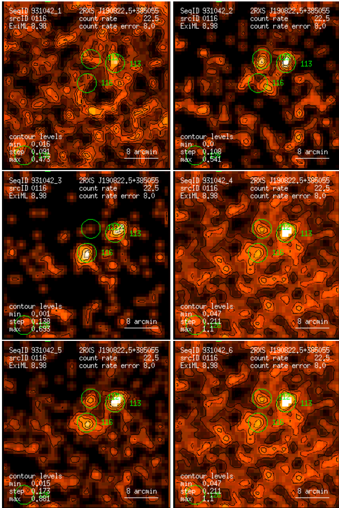
Figure 116: RASS 931042: detection 0116: band rate images, Gaussian filter: (1) PSPC channels 11 – 41, (2) 52 – 90, (3) 91 – 201, (4) 11 – 235, (5) 52 – 201, (6) 11 – 201. Broad band rates in counts/ks. Band rate contour levels in counts/ks/arcmin 2 .
