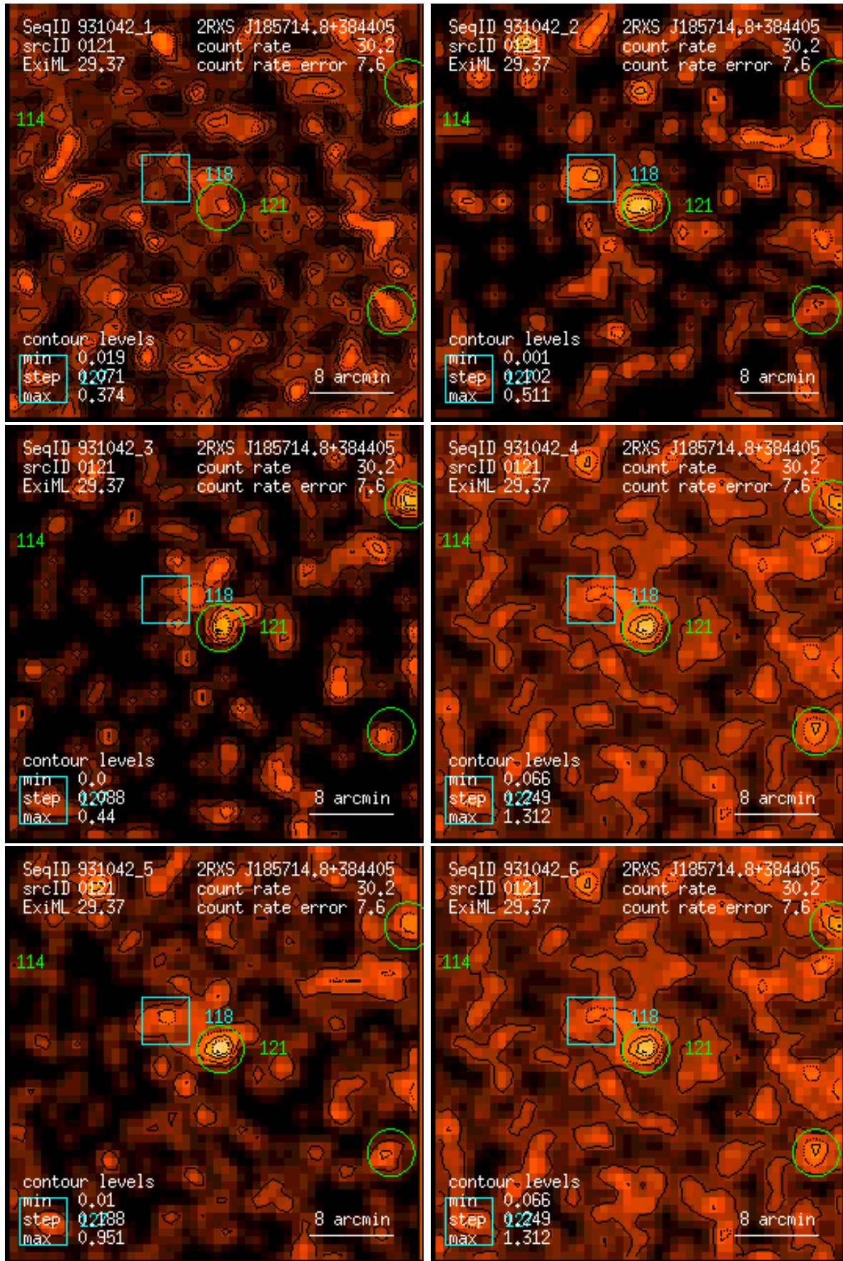
Figure 121: RASS 931042: detection 0121: band rate images, Gaussian filter: (1) PSPC channels 11 – 41, (2) 52 – 90, (3) 91 – 201, (4) 11 – 235, (5) 52 – 201, (6) 11 – 201. Broad band rates in counts/ks. Band rate contour levels in counts/ks/arcmin 2 .
