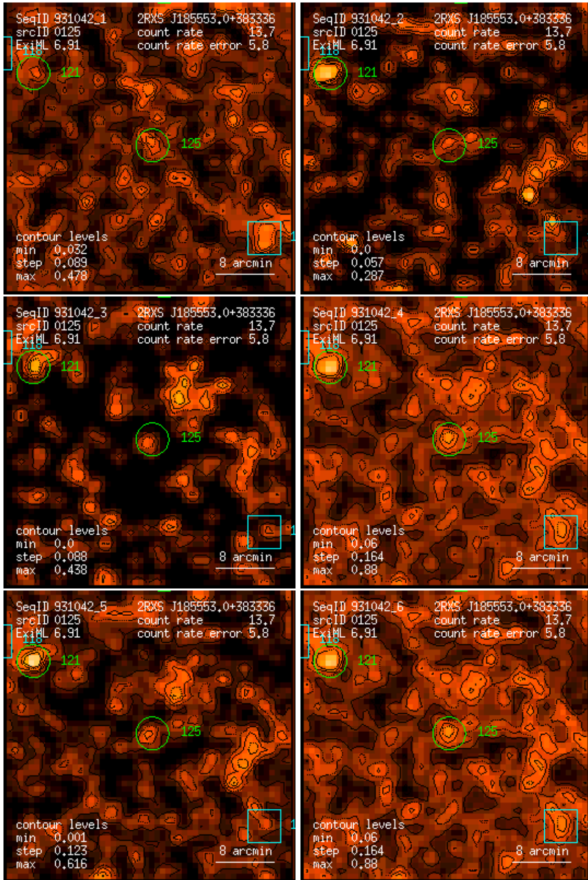
Figure 125: RASS 931042: detection 0125: band rate images, Gaussian filter: (1) PSPC channels 11 – 41, (2) 52 – 90, (3) 91 – 201, (4) 11 – 235, (5) 52 – 201, (6) 11 – 201. Broad band rates in counts/ks. Band rate contour levels in counts/ks/arcmin 2 .
