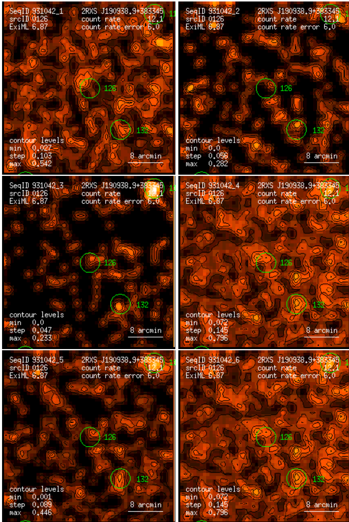
Figure 126: RASS 931042: detection 0126: band rate images, Gaussian filter: (1) PSPC channels 11 – 41, (2) 52 – 90, (3) 91 – 201, (4) 11 – 235, (5) 52 – 201, (6) 11 – 201. Broad band rates in counts/ks. Band rate contour levels in counts/ks/arcmin 2 .
