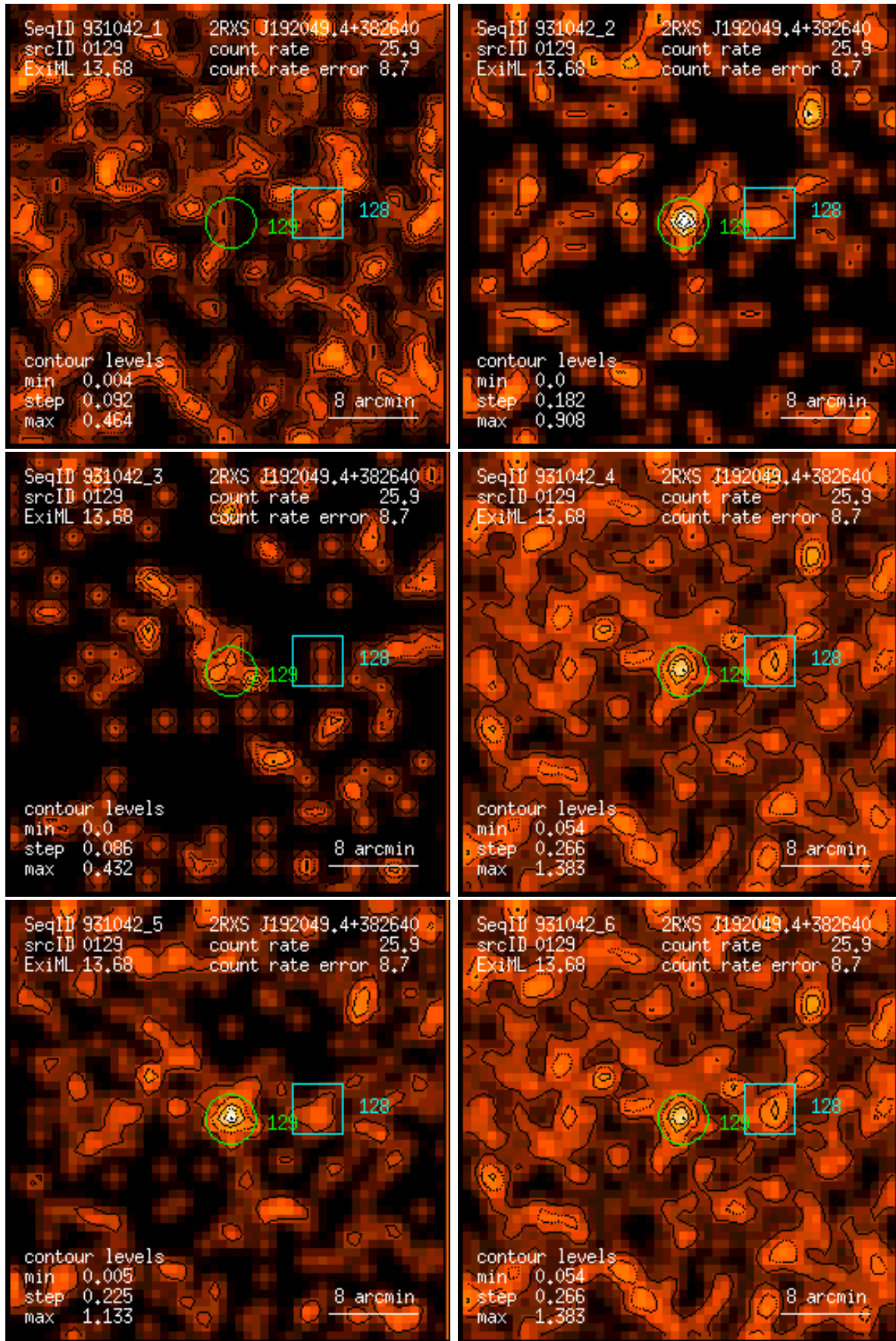
Figure 129: RASS 931042: detection 0129: band rate images, Gaussian filter: (1) PSPC channels 11 – 41, (2) 52 – 90, (3) 91 – 201, (4) 11 – 235, (5) 52 – 201, (6) 11 – 201. Broad band rates in counts/ks. Band rate contour levels in counts/ks/arcmin 2 .
