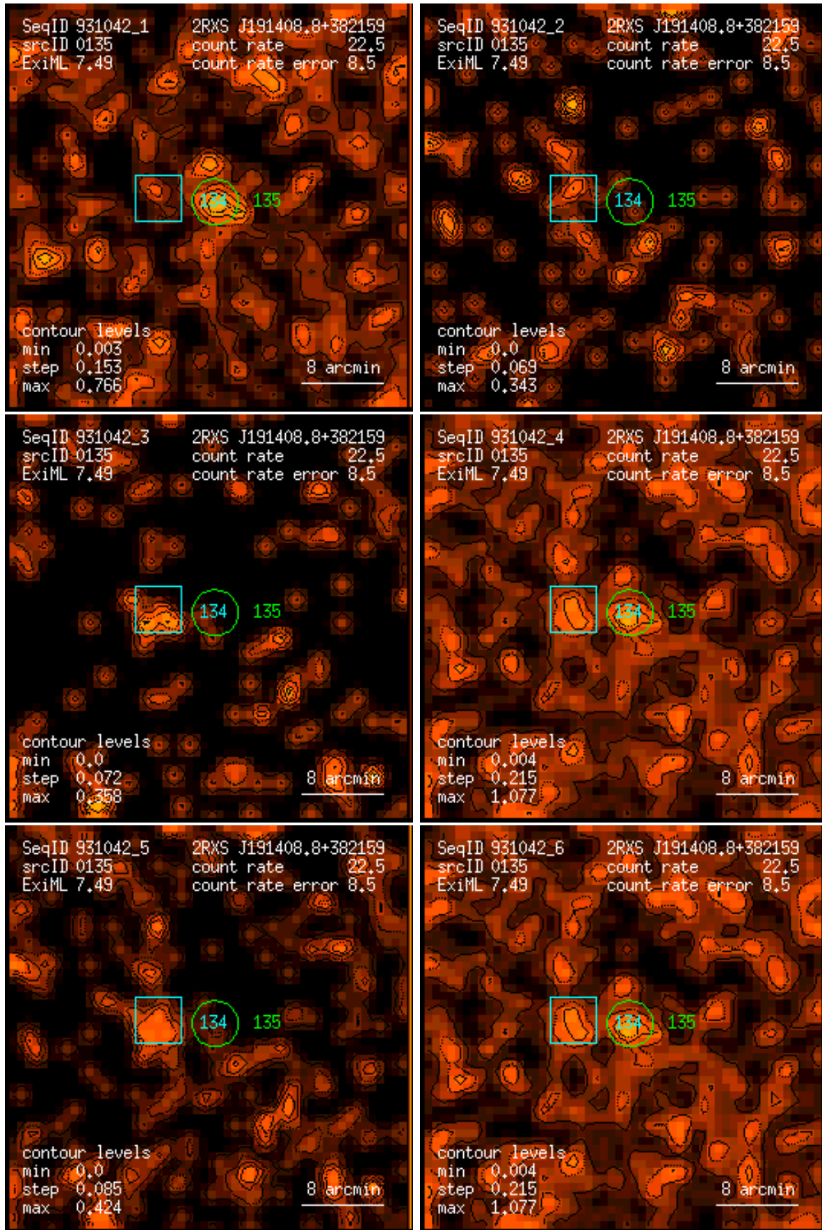
Figure 135: RASS 931042: detection 0135: band rate images, Gaussian filter: (1) PSPC channels 11 – 41, (2) 52 – 90, (3) 91 – 201, (4) 11 – 235, (5) 52 – 201, (6) 11 – 201. Broad band rates in counts/ks. Band rate contour levels in counts/ks/arcmin 2 .
