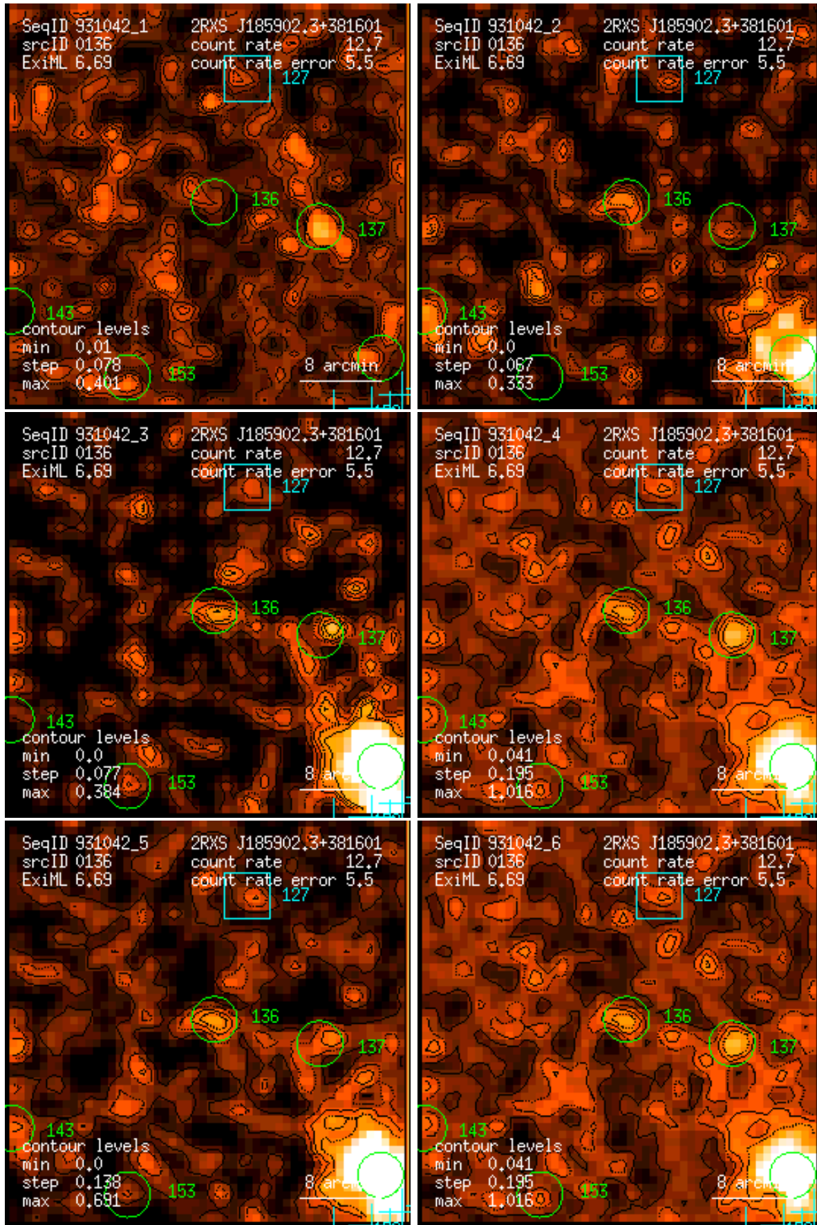
Figure 136: RASS 931042: detection 0136: band rate images, Gaussian filter: (1) PSPC channels 11 – 41, (2) 52 – 90, (3) 91 – 201, (4) 11 – 235, (5) 52 – 201, (6) 11 – 201. Broad band rates in counts/ks. Band rate contour levels in counts/ks/arcmin 2 .
