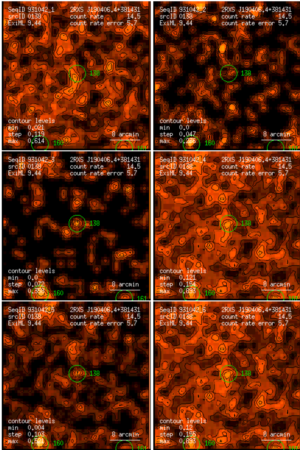
Figure 138: RASS 931042: detection 0138: band rate images, Gaussian filter: (1) PSPC channels 11 – 41, (2) 52 – 90, (3) 91 – 201, (4) 11 – 235, (5) 52 – 201, (6) 11 – 201. Broad band rates in counts/ks. Band rate contour levels in counts/ks/arcmin 2 .
