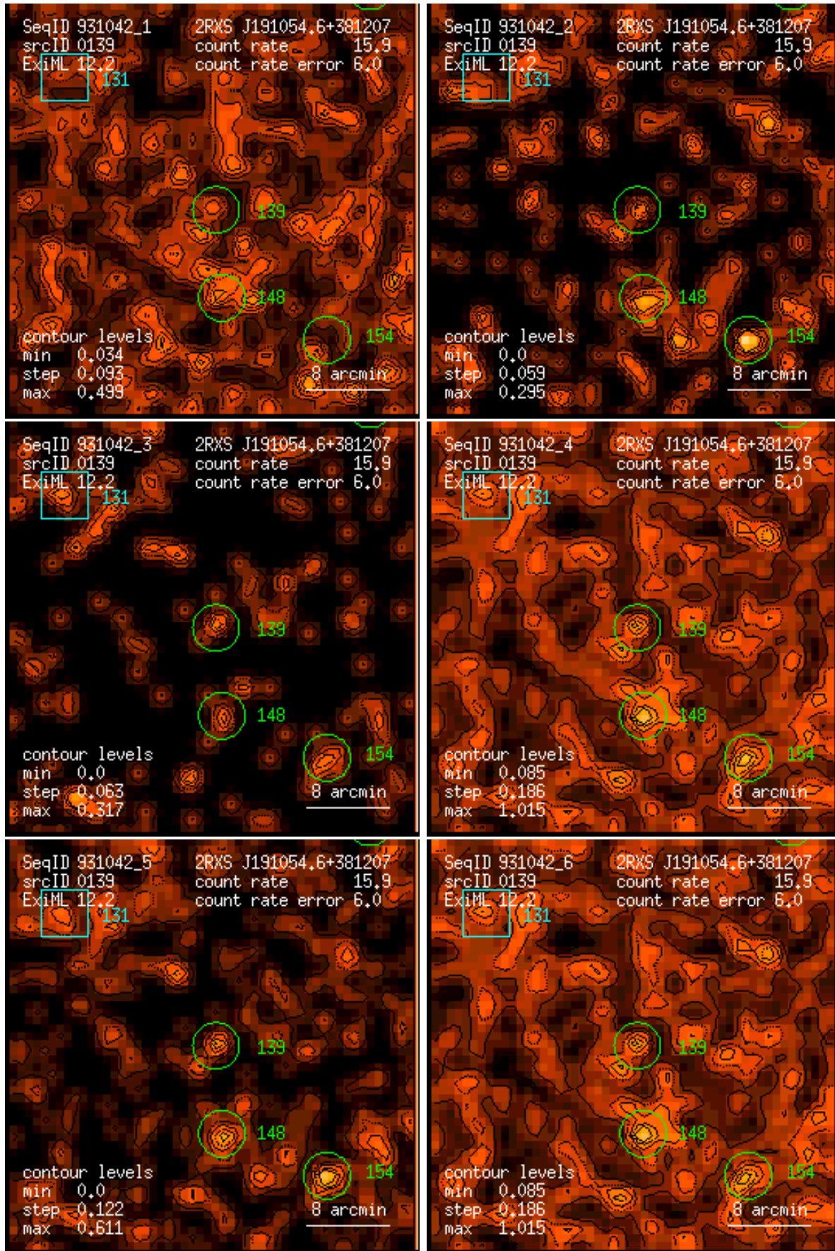
Figure 139: RASS 931042: detection 0139: band rate images, Gaussian filter: (1) PSPC channels 11 – 41, (2) 52 – 90, (3) 91 – 201, (4) 11 – 235, (5) 52 – 201, (6) 11 – 201. Broad band rates in counts/ks. Band rate contour levels in counts/ks/arcmin 2 .
