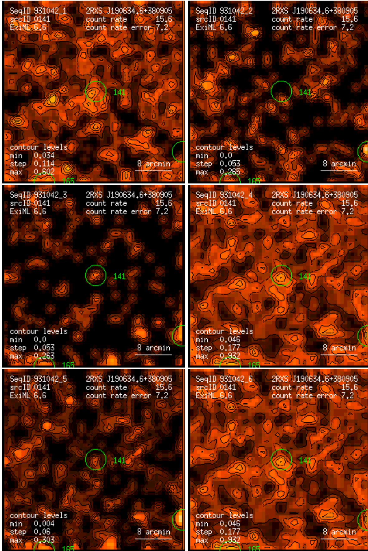
Figure 141: RASS 931042: detection 0141: band rate images, Gaussian filter: (1) PSPC channels 11 – 41, (2) 52 – 90, (3) 91 – 201, (4) 11 – 235, (5) 52 – 201, (6) 11 – 201. Broad band rates in counts/ks. Band rate contour levels in counts/ks/arcmin 2 .
