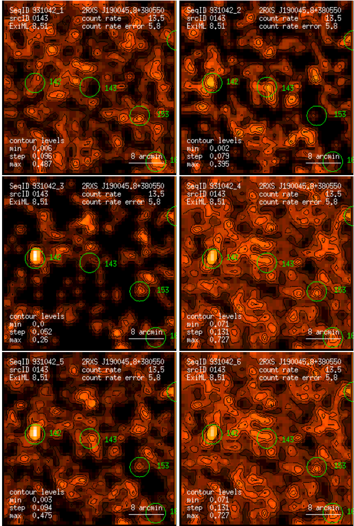
Figure 143: RASS 931042: detection 0143: band rate images, Gaussian filter: (1) PSPC channels 11 – 41, (2) 52 – 90, (3) 91 – 201, (4) 11 – 235, (5) 52 – 201, (6) 11 – 201. Broad band rates in counts/ks. Band rate contour levels in counts/ks/arcmin 2 .
