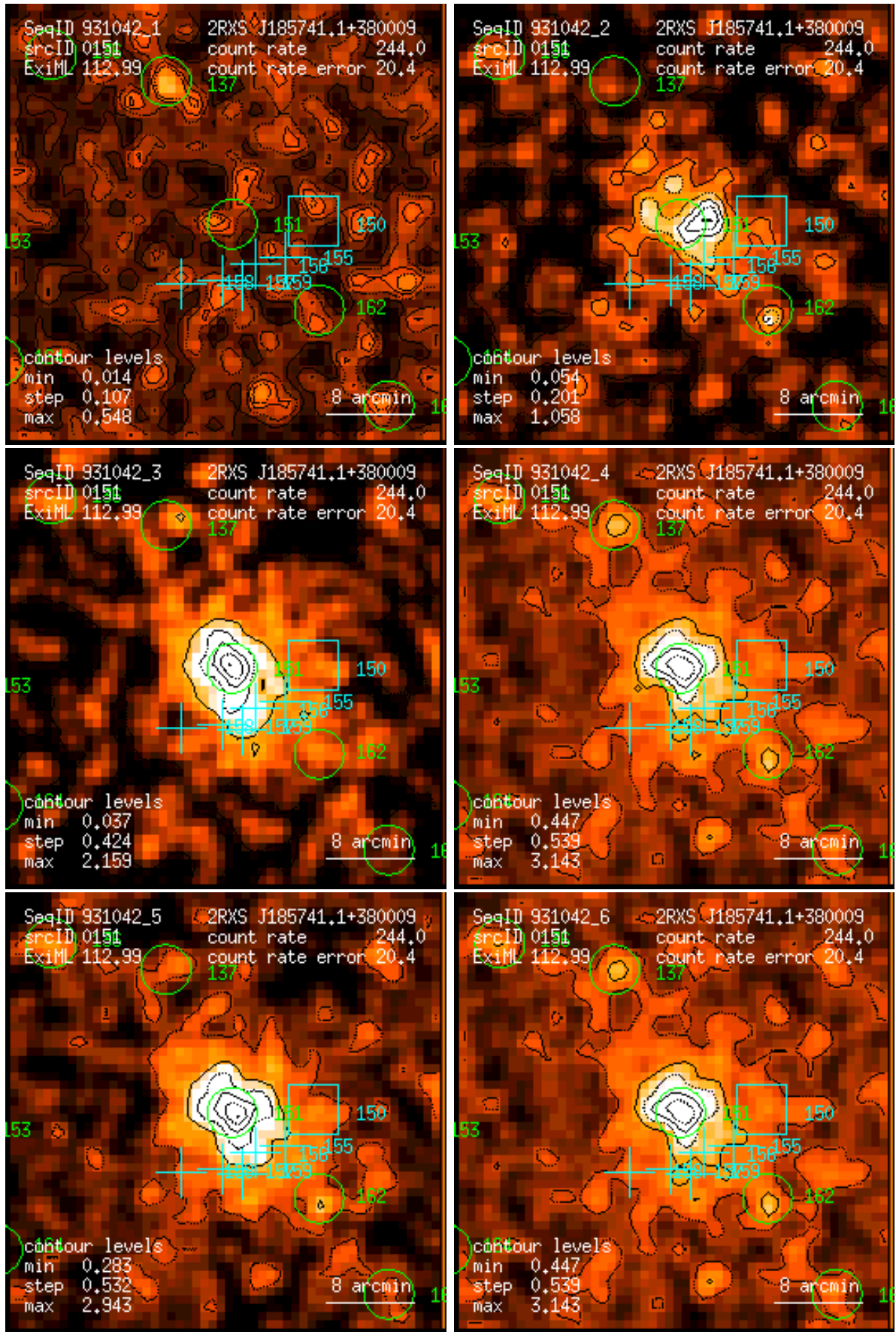
Figure 151: RASS 931042: detection 0151: band rate images, Gaussian filter: (1) PSPC channels 11 – 41, (2) 52 – 90, (3) 91 – 201, (4) 11 – 235, (5) 52 – 201, (6) 11 – 201. Broad band rates in counts/ks. Band rate contour levels in counts/ks/arcmin 2 .
