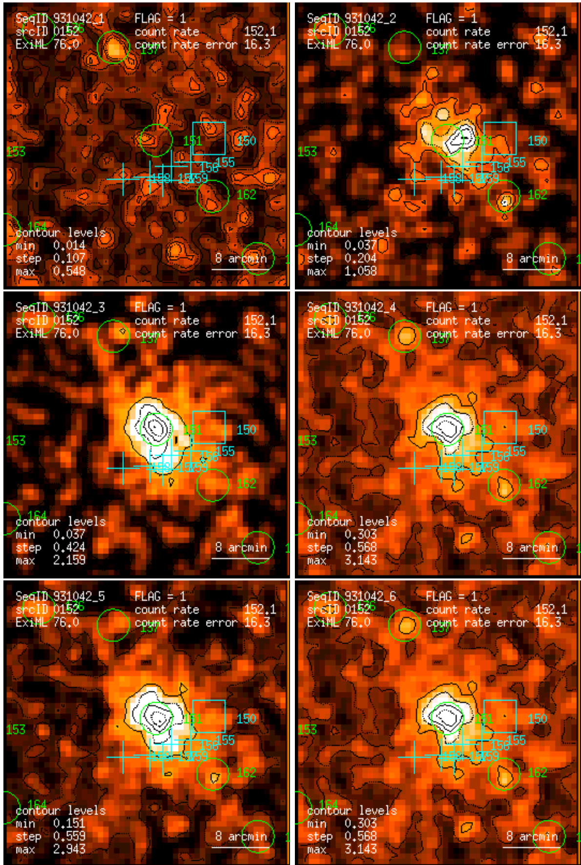
Figure 152: RASS 931042: detection 0152: band rate images, Gaussian filter: (1) PSPC channels 11 – 41, (2) 52 – 90, (3) 91 – 201, (4) 11 – 235, (5) 52 – 201, (6) 11 – 201. Broad band rates in counts/ks. Band rate contour levels in counts/ks/arcmin 2 .
