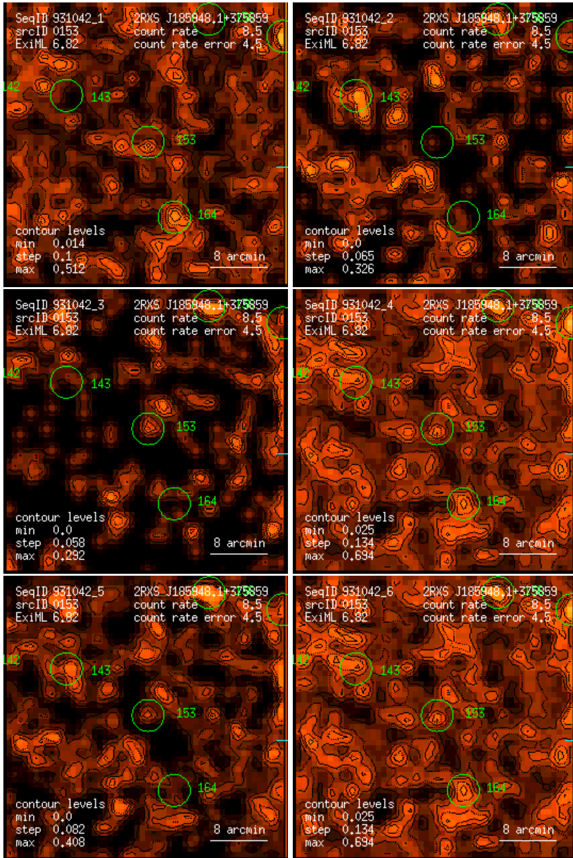
Figure 153: RASS 931042: detection 0153: band rate images, Gaussian filter: (1) PSPC channels 11 – 41, (2) 52 – 90, (3) 91 – 201, (4) 11 – 235, (5) 52 – 201, (6) 11 – 201. Broad band rates in counts/ks. Band rate contour levels in counts/ks/arcmin 2 .
