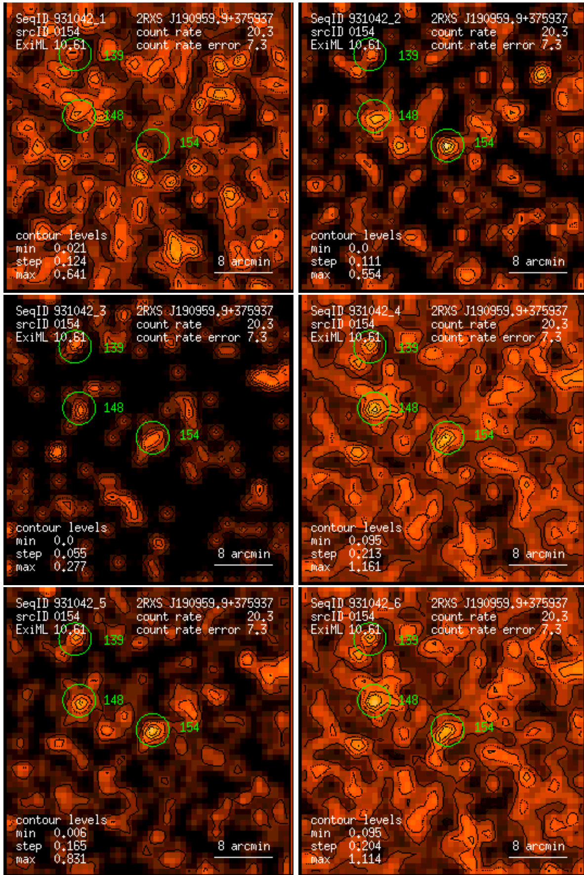
Figure 154: RASS 931042: detection 0154: band rate images, Gaussian filter: (1) PSPC channels 11 – 41, (2) 52 – 90, (3) 91 – 201, (4) 11 – 235, (5) 52 – 201, (6) 11 – 201. Broad band rates in counts/ks. Band rate contour levels in counts/ks/arcmin 2 .
