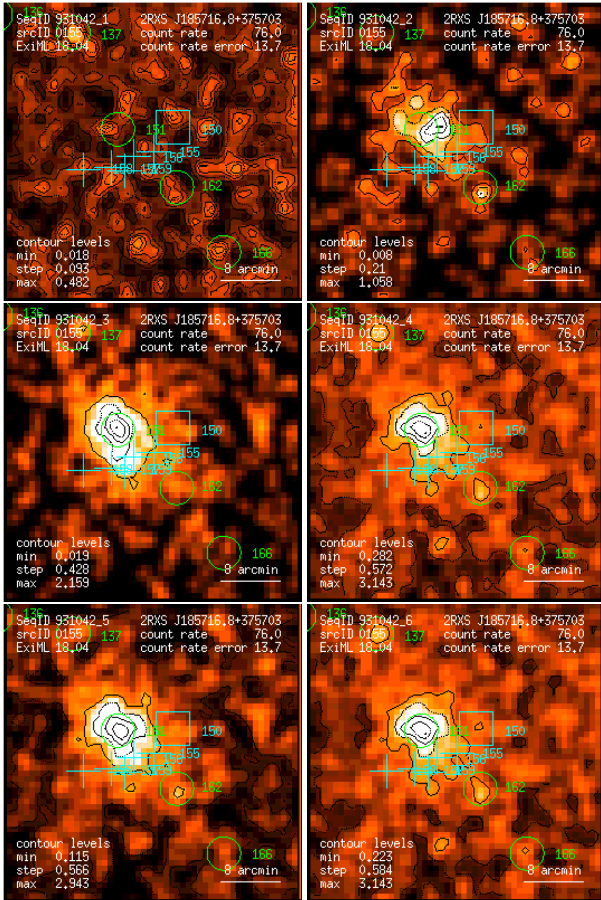
Figure 155: RASS 931042: detection 0155: band rate images, Gaussian filter: (1) PSPC channels 11 – 41, (2) 52 – 90, (3) 91 – 201, (4) 11 – 235, (5) 52 – 201, (6) 11 – 201. Broad band rates in counts/ks. Band rate contour levels in counts/ks/arcmin 2 .
