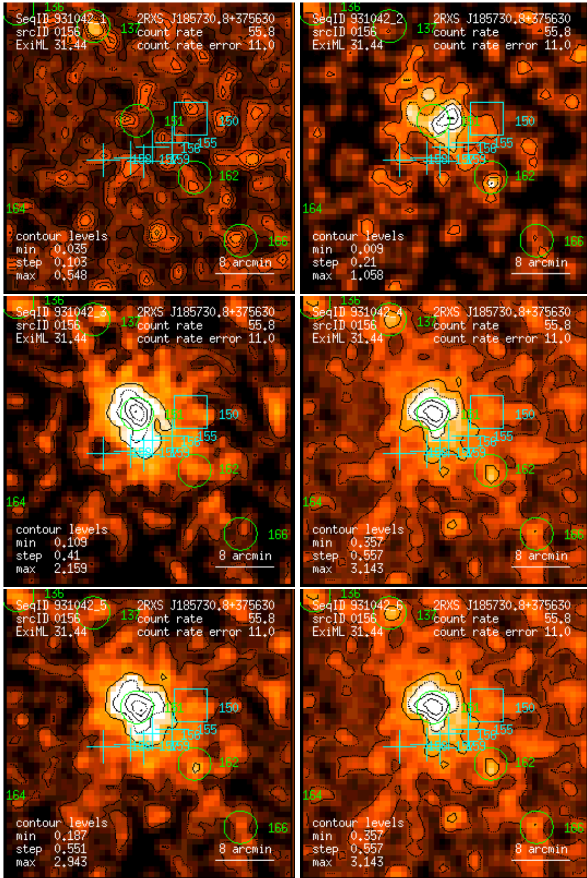
Figure 156: RASS 931042: detection 0156: band rate images, Gaussian filter: (1) PSPC channels 11 – 41, (2) 52 – 90, (3) 91 – 201, (4) 11 – 235, (5) 52 – 201, (6) 11 – 201. Broad band rates in counts/ks. Band rate contour levels in counts/ks/arcmin 2 .
