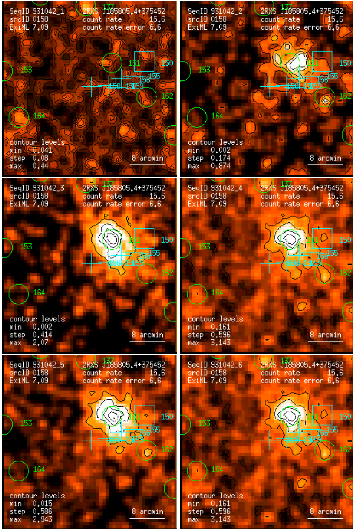
Figure 158: RASS 931042: detection 0158: band rate images, Gaussian filter: (1) PSPC channels 11 – 41, (2) 52 – 90, (3) 91 – 201, (4) 11 – 235, (5) 52 – 201, (6) 11 – 201. Broad band rates in counts/ks. Band rate contour levels in counts/ks/arcmin 2 .
