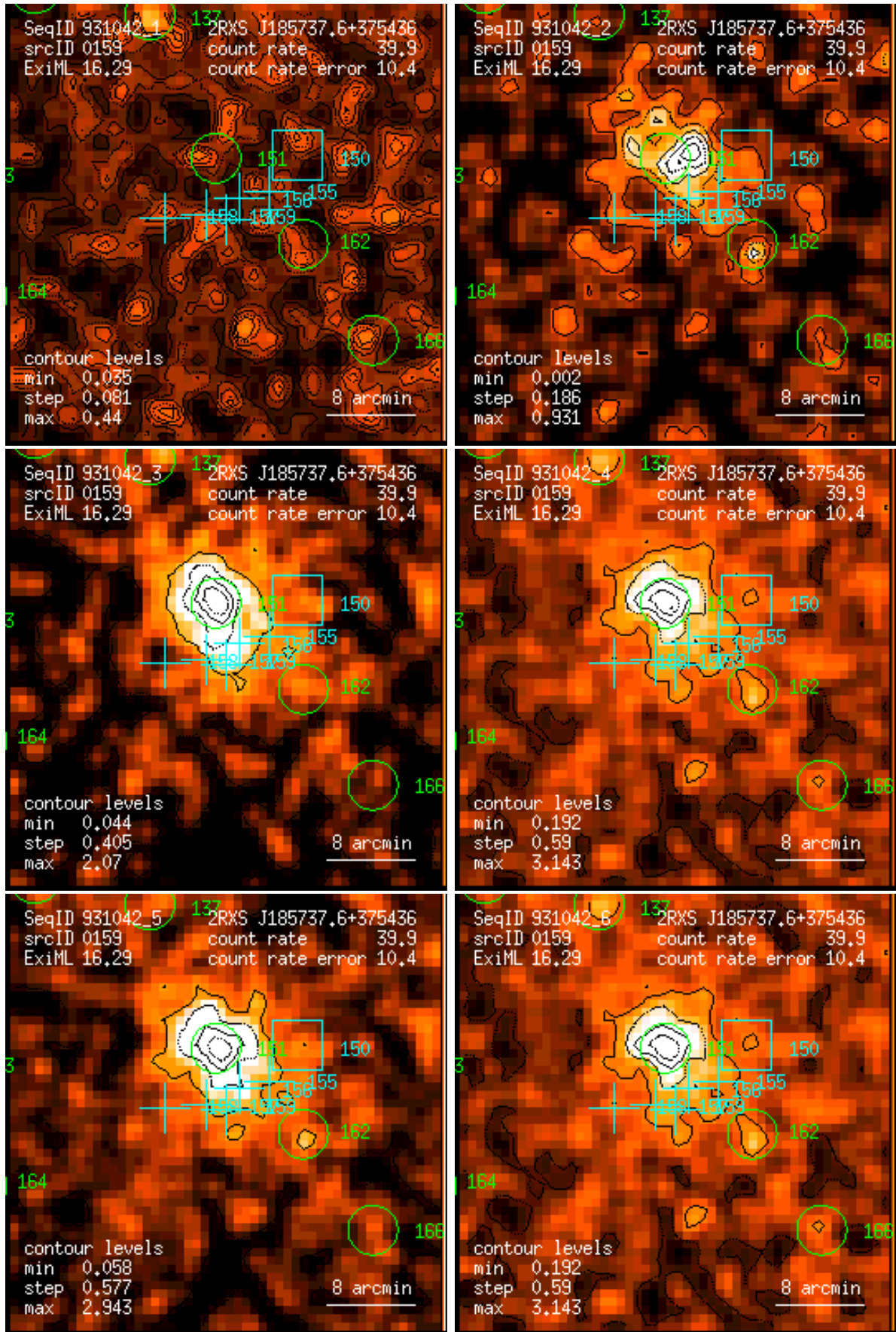
Figure 159: RASS 931042: detection 0159: band rate images, Gaussian filter: (1) PSPC channels 11 – 41, (2) 52 – 90, (3) 91 – 201, (4) 11 – 235, (5) 52 – 201, (6) 11 – 201. Broad band rates in counts/ks. Band rate contour levels in counts/ks/arcmin 2 .
