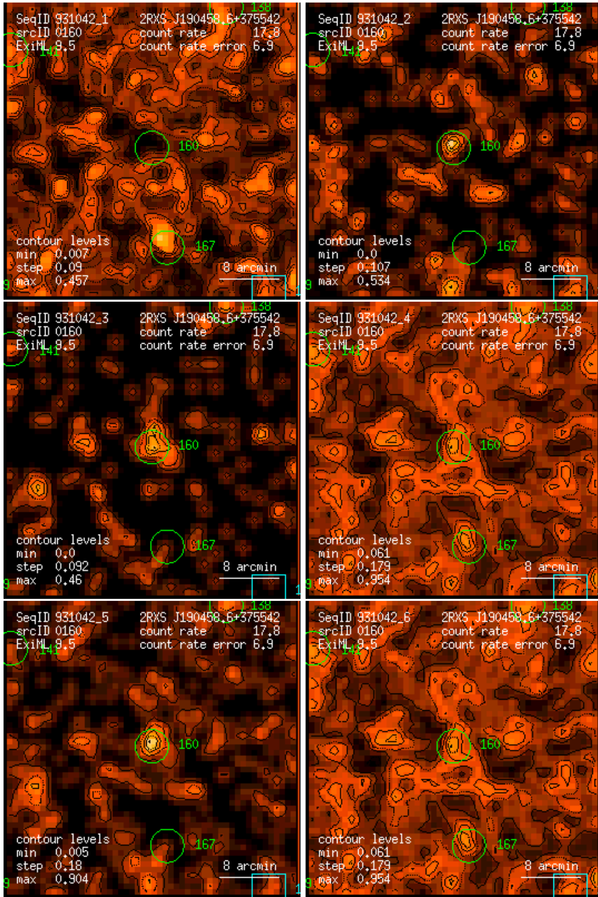
Figure 160: RASS 931042: detection 0160: band rate images, Gaussian filter: (1) PSPC channels 11 – 41, (2) 52 – 90, (3) 91 – 201, (4) 11 – 235, (5) 52 – 201, (6) 11 – 201. Broad band rates in counts/ks. Band rate contour levels in counts/ks/arcmin 2 .
