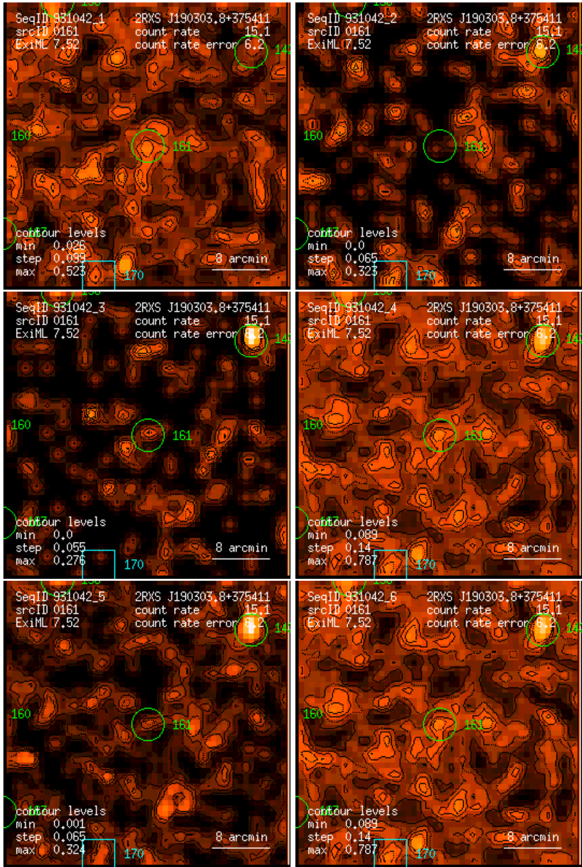
Figure 161: RASS 931042: detection 0161: band rate images, Gaussian filter: (1) PSPC channels 11 – 41, (2) 52 – 90, (3) 91 – 201, (4) 11 – 235, (5) 52 – 201, (6) 11 – 201. Broad band rates in counts/ks. Band rate contour levels in counts/ks/arcmin 2 .
