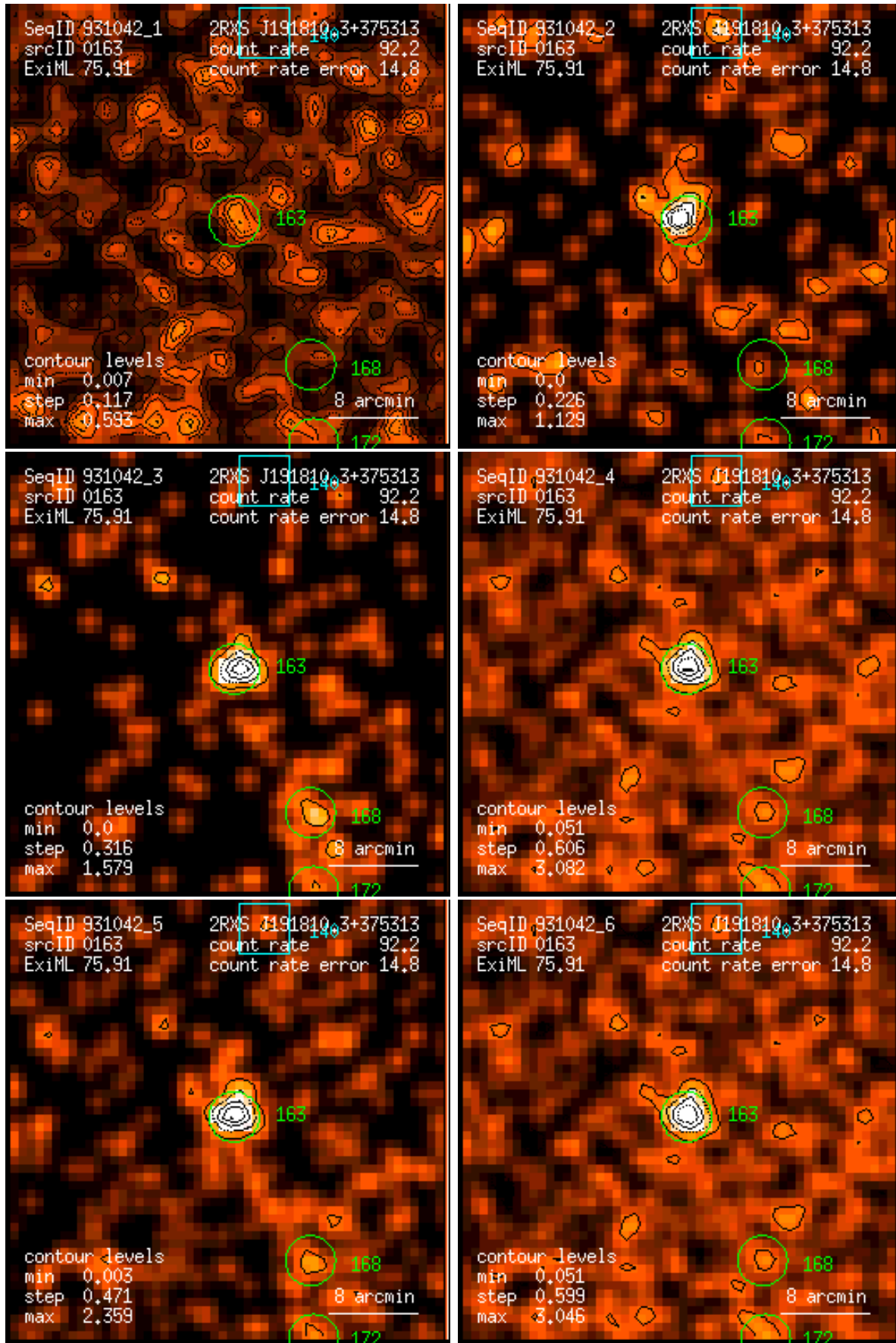
Figure 163: RASS 931042: detection 0163: band rate images, Gaussian filter: (1) PSPC channels 11 – 41, (2) 52 – 90, (3) 91 – 201, (4) 11 – 235, (5) 52 – 201, (6) 11 – 201. Broad band rates in counts/ks. Band rate contour levels in counts/ks/arcmin 2 .
