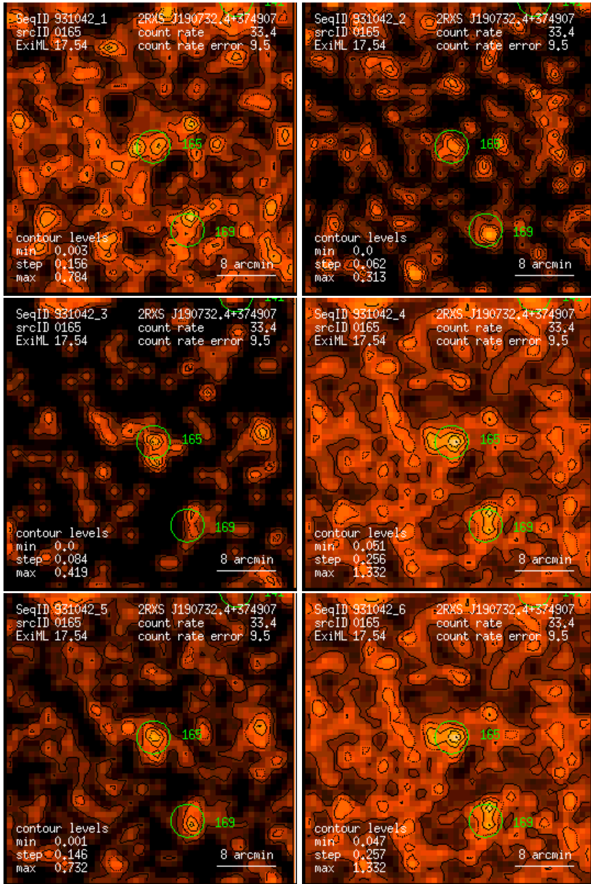
Figure 165: RASS 931042: detection 0165: band rate images, Gaussian filter: (1) PSPC channels 11 – 41, (2) 52 – 90, (3) 91 – 201, (4) 11 – 235, (5) 52 – 201, (6) 11 – 201. Broad band rates in counts/ks. Band rate contour levels in counts/ks/arcmin 2 .
