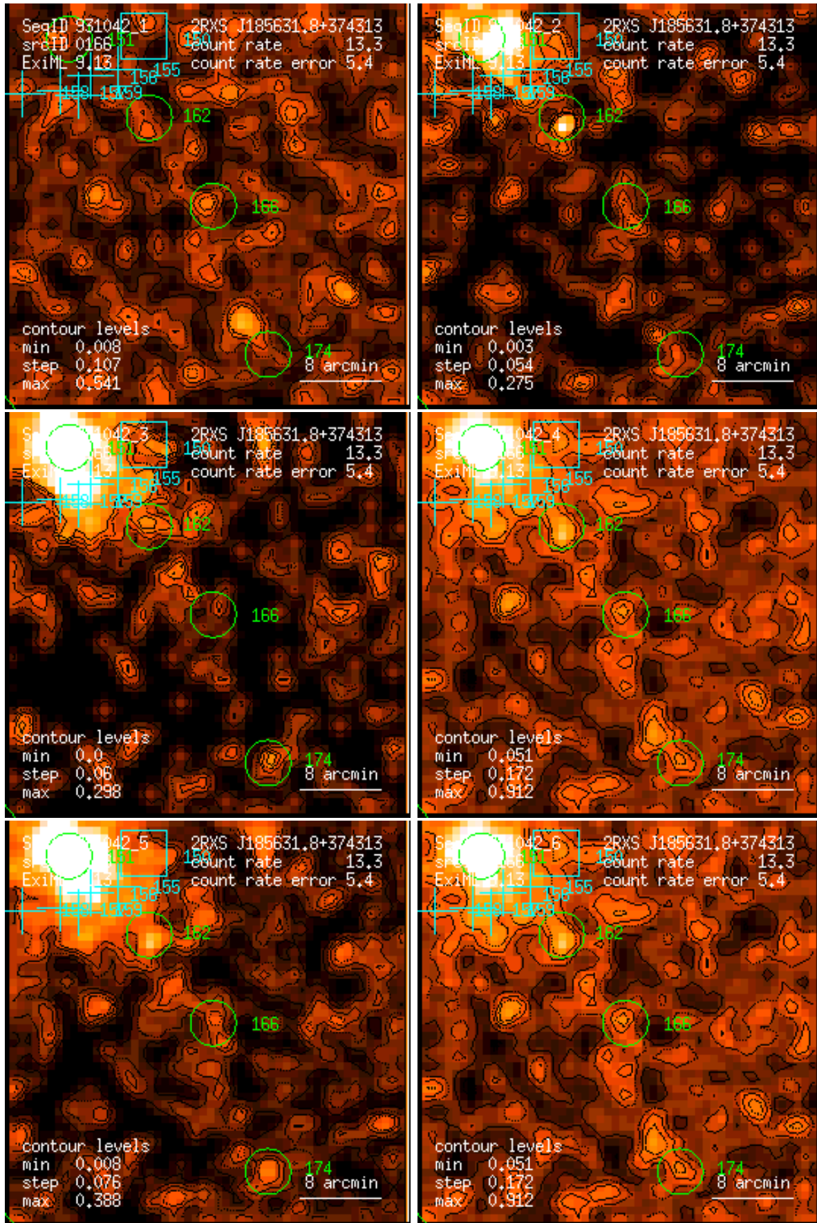
Figure 166: RASS 931042: detection 0166: band rate images, Gaussian filter: (1) PSPC channels 11 – 41, (2) 52 – 90, (3) 91 – 201, (4) 11 – 235, (5) 52 – 201, (6) 11 – 201. Broad band rates in counts/ks. Band rate contour levels in counts/ks/arcmin 2 .
