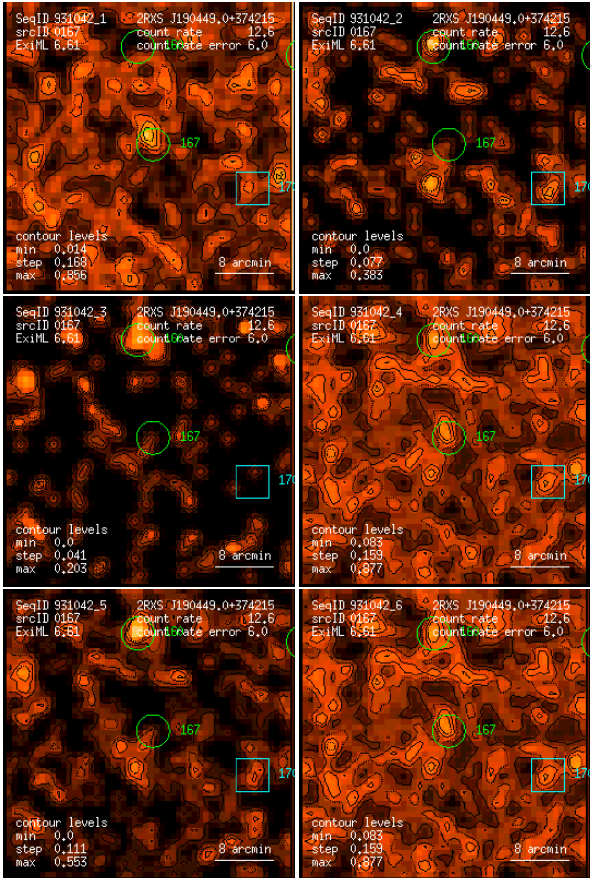
Figure 167: RASS 931042: detection 0167: band rate images, Gaussian filter: (1) PSPC channels 11 – 41, (2) 52 – 90, (3) 91 – 201, (4) 11 – 235, (5) 52 – 201, (6) 11 – 201. Broad band rates in counts/ks. Band rate contour levels in counts/ks/arcmin 2 .
