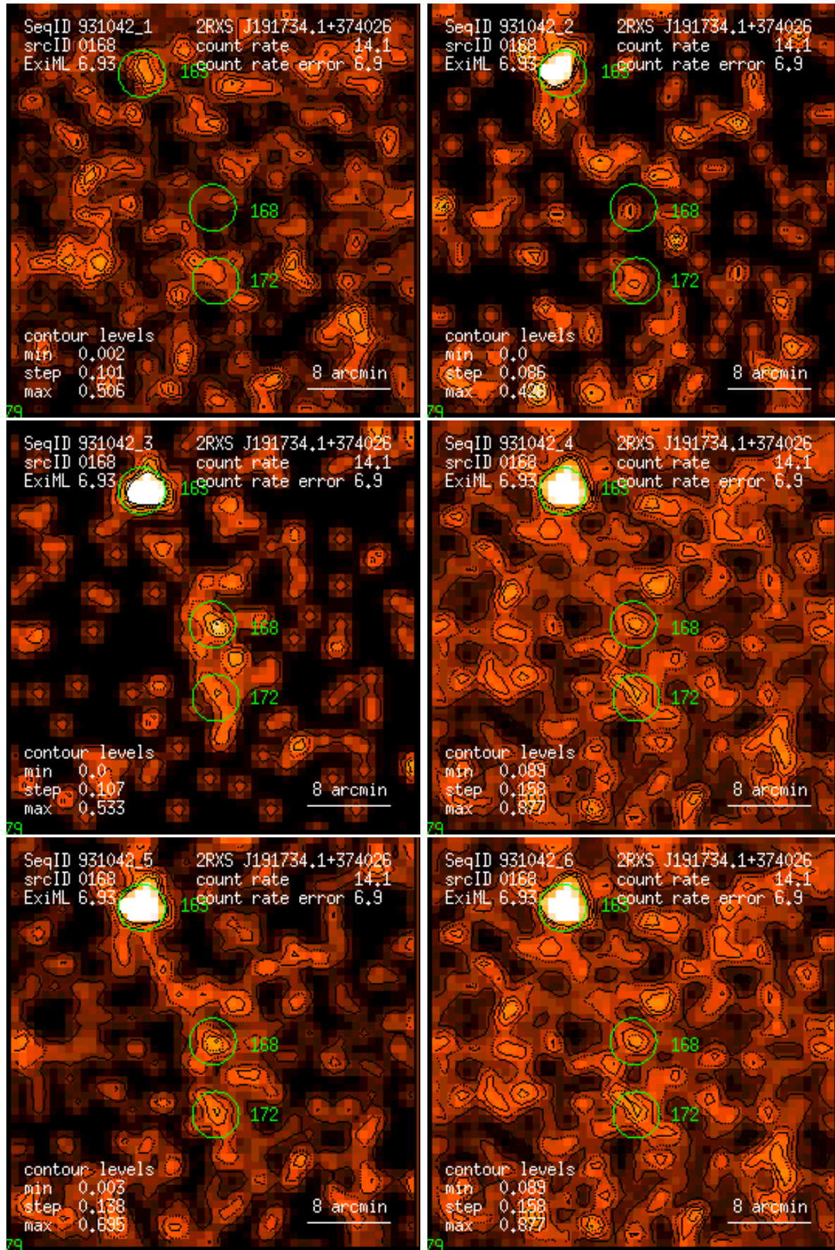
Figure 168: RASS 931042: detection 0168: band rate images, Gaussian filter: (1) PSPC channels 11 – 41, (2) 52 – 90, (3) 91 – 201, (4) 11 – 235, (5) 52 – 201, (6) 11 – 201. Broad band rates in counts/ks. Band rate contour levels in counts/ks/arcmin 2 .
